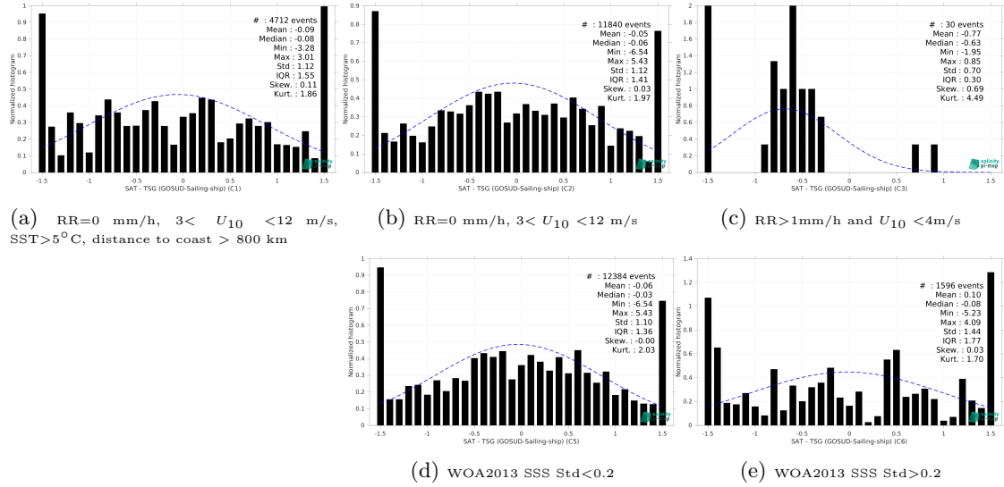
Figure 15: Normalized histogram of \Delta SSS (SMOS SSS L2Q v331 - No FLAG (CMEMS-CATDS-CPDC) - TSG (GOSUD-Sailing-ship)) for 5 different subdatasets corresponding to: RR=0 mm/h, 3 < U_{10} < 12 m/s, SST > 5°C, distance to coast > 800 km (a), RR=0 mm/h, 3 < U_{10} < 12 m/s (b), RR > 1mm/h and U_{10} < 4 m/s (c), WOA2013 SSS Std < 0.2 (d), WOA2013 SSS Std > 0.2 (e).
