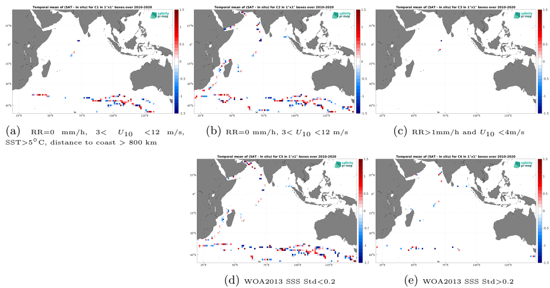
Figure 14: Temporal mean gridded over spatial boxes of size 1^\circ \times 1^\circ of \Delta SSS (SMOS SSS L2Q v331 - No FLAG (CMEMS-CATDS-CPDC) - TSG (GOSUD-Sailing-ship)) for 5 different sub-datasets corresponding to:RR=0 mm/h, 3 < U_{10} < 12 m/s, SST >5^\circ C, distance to coast > 800 km (a), RR=0 mm/h, 3 < U_{10} < 12 m/s (b), RR >1 mm/h and U_{10} < 4 m/s (c), WOA2013 SSS Std <0.2 (d), WOA2013 SSS Std >0.2 (e).
