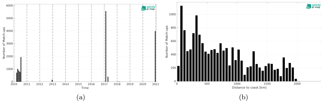
Figure 2: Number of match-ups between TSG (GOSUD-Sailing-ship) and SMOS SSS L2Q v331 - No FLAG (CMEMS-CATDS-CPDC) SSS as a function of time (a) and as function of the distance to coast (b) over the Indian Ocean Pi-MEP region and for the full satellite product period.
