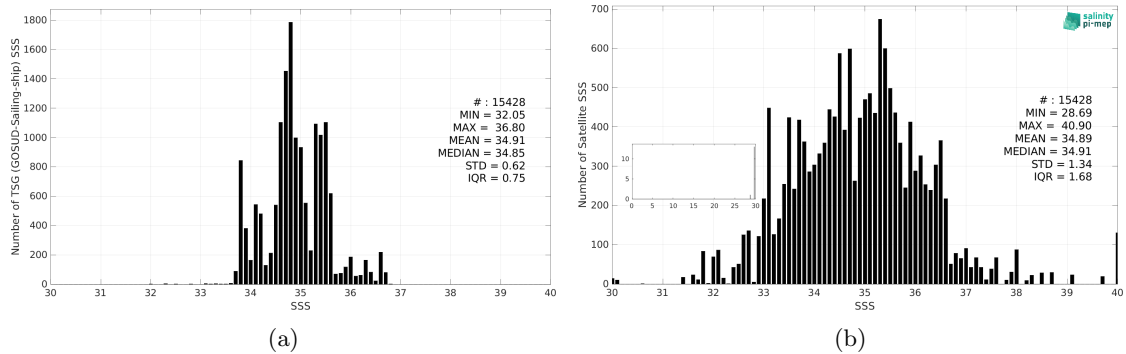
Figure 3: Histograms of SSS from TSG (GOSUD-Sailing-ship) (a) and SMOS SSS L2Q v331 - No FLAG (CMEMS-CATDS-CPDC) (b) considering all match-up pairs per bins of 0.1 over the Indian Ocean Pi-MEP region and for the full satellite product period.
