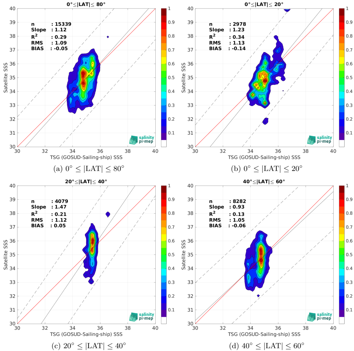
Figure 10: Contour maps of the concentration of SMOS SSS L2Q v331 - No FLAG (CMEMS-CATDS-CPDC) SSS (y-axis) versus TSG (GOSUD-Sailing-ship) SSS (x-axis) at match-up pairs for different latitude bands. For each plot, the red line shows x=y . The black thin and dashed lines indicate a linear fit through the data cloud and the \pm 95\% confidence levels, respectively. The number match-up pairs n , the slope and R^2 coefficient of the linear fit, the root mean square (RMS) and the mean bias between satellite and in situ data are indicated for each latitude band in each plots.
