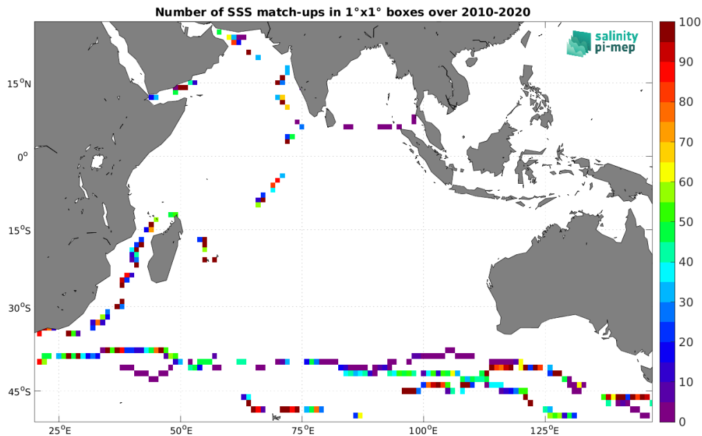
Figure 5: Number of SSS match-ups between TSG (GOSUD-Sailing-ship) SSS and the SMOS SSS L2Q v331 - No FLAG (CMEMS-CATDS-CPDC) SSS product for the Indian Ocean Pi-MEP region over 1^\circ \times 1^\circ boxes and for the full satellite product period.
