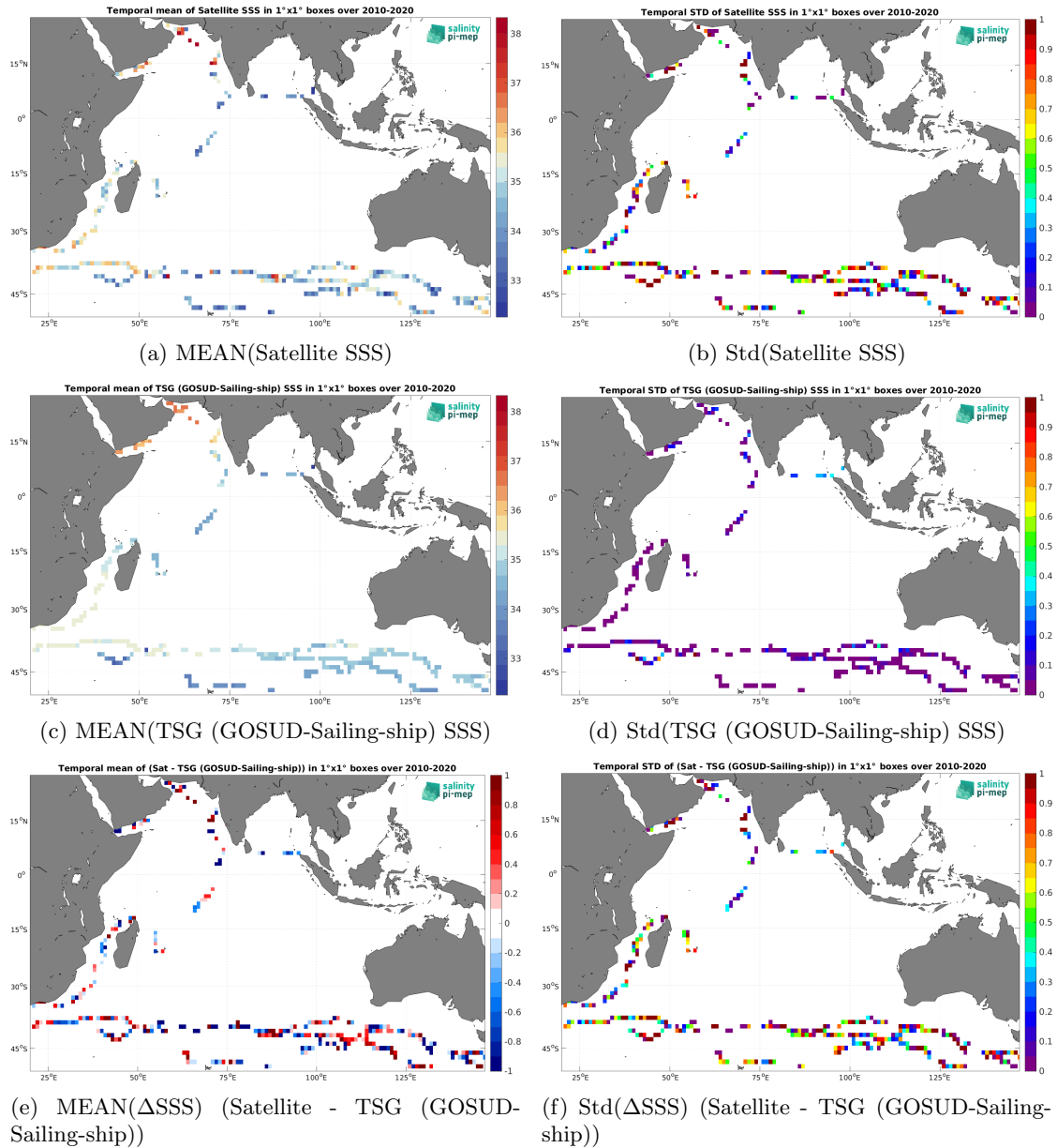
Figure 7: Temporal mean (left) and Std (right) of SSS from SMOS SSS L2Q v331 - No FLAG (CMEMS-CATDS-CPDC) (top), TSG (GOSUD-Sailing-ship) (middle), and of \Delta SSS (Satellite - TSG (GOSUD-Sailing-ship)). Only match-up pairs are used to generate these maps.
