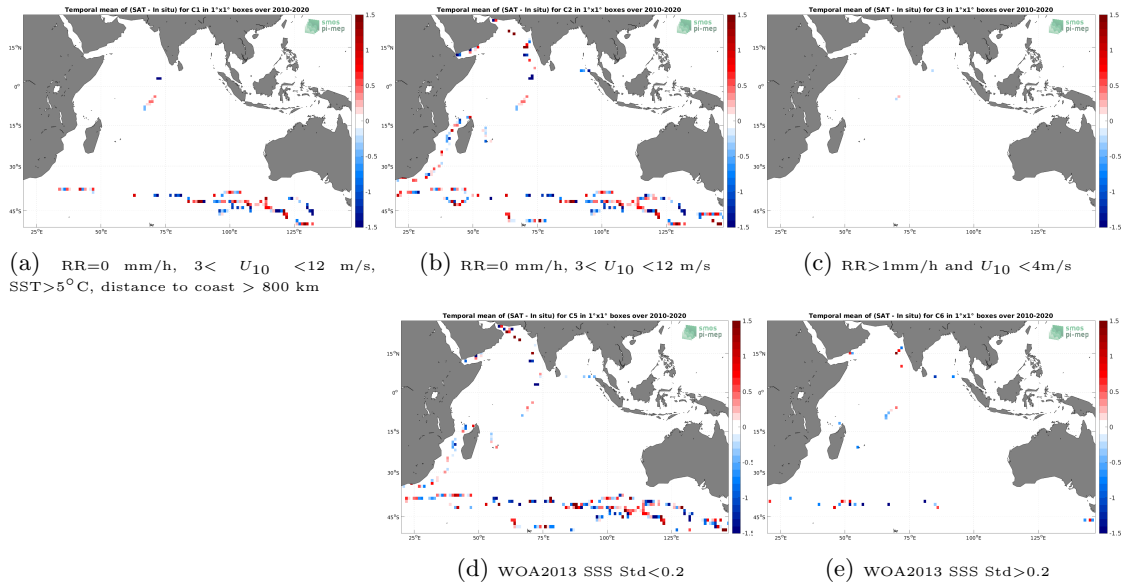
Figure 12: Temporal mean gridded over spatial boxes of size 1^\circ \times 1^\circ of \Delta SSS (SMOS SSS L2Q v331 - No FLAG (CMEMS-CATDS-CPDC) - TSG (GOSUD-Sailing-ship)) for 5 different sub-datasets corresponding to:RR=0 mm/h, 3 < U_{10} < 12 m/s, SST > 5^\circ\text{C} , distance to coast > 800 km (a), RR=0 mm/h, 3 < U_{10} < 12 m/s (b), RR > 1 mm/h and U_{10} < 4 m/s (c), WOA2013 SSS Std < 0.2 (d), WOA2013 SSS Std > 0.2 (e).
