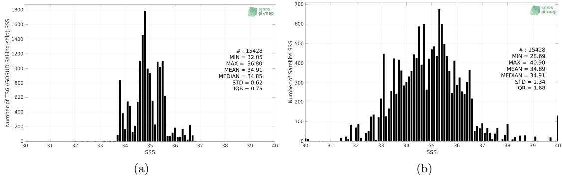
Figure 2: Histograms of SSS from TSG (GOSUD-Sailing-ship) (a) and SMOS SSS L2Q v331 - No FLAG (CMEMS-CATDS-CPDC) (b) considering all match-up pairs per bins of 0.1 over the Indian Ocean Pi-MEP region and for the full satellite product period.
