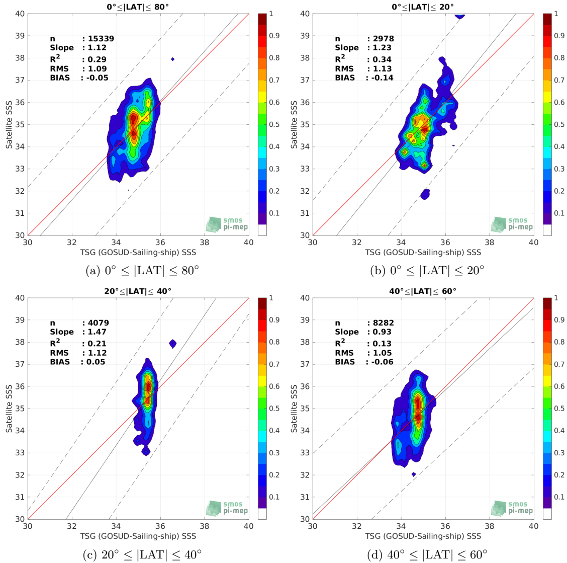
Figure 9: Contour maps of the concentration of SMOS SSS L2Q v331 - No FLAG (CMEMS-CATDS-CPDC) SSS (y-axis) versus TSG (GOSUD-Sailing-ship) SSS (x-axis) at match-up pairs for different latitude bands. For each plot, the red line shows x=y . The black thin and dashed lines indicate a linear fit through the data cloud and the \pm 95\% confidence levels, respectively. The number match-up pairs n , the slope and R^2 coefficient of the linear fit, the root mean square (RMS) and the mean bias between satellite and in situ data are indicated for each latitude band in each plots.
