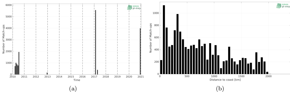
Figure 1: Number of match-ups between TSG (GOSUD-Sailing-ship) and SMOS SSS L2Q v331 - No FLAG (CMEMS-CATDS-CPDC) SSS as a function of time (a) and as function of the distance to coast (b) over the Indian Ocean Pi-MEP region and for the full satellite product period.
