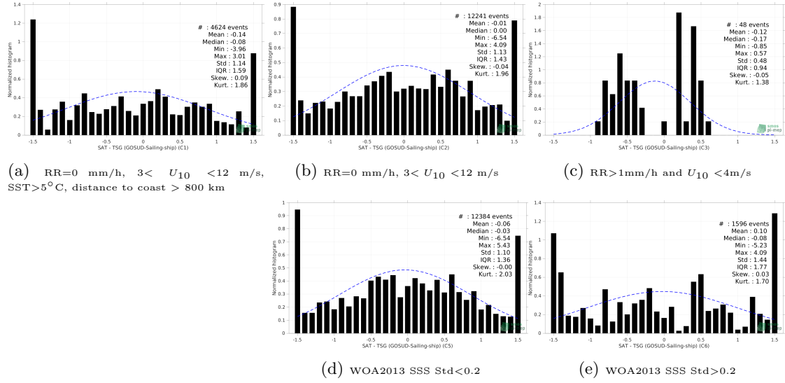
Figure 13: Normalized histogram of \Delta SSS (SMOS SSS L2Q v331 - No FLAG (CMEMS-CATDS-CPDC) - TSG (GOSUD-Sailing-ship)) for 5 different subdatasets corresponding to: RR=0 mm/h, 3 < U_{10} < 12 m/s, SST>5°C, distance to coast > 800 km (a), RR=0 mm/h, 3 < U_{10} < 12 m/s (b), RR>1mm/h and U_{10} < 4 m/s (c), WOA2013 SSS Std<0.2 (d), WOA2013 SSS Std>0.2 (e).
