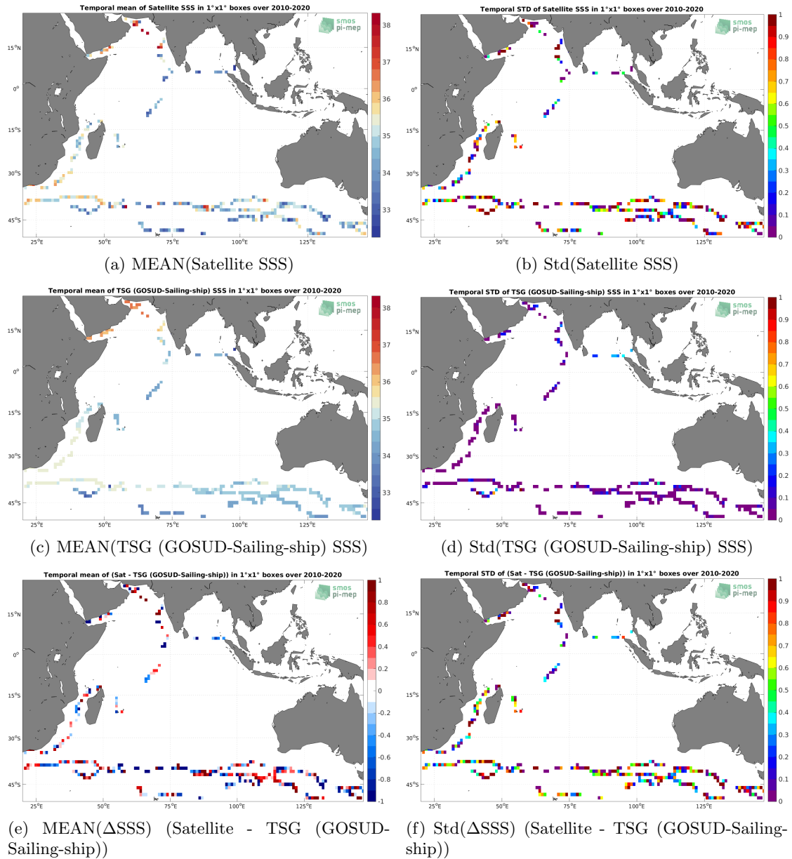
Figure 6: Temporal mean (left) and Std (right) of SSS from SMOS SSS L2Q v331 - No FLAG (CMEMS-CATDS-CPDC) (top), TSG (GOSUD-Sailing-ship) (middle), and of \Delta SSS (Satellite - TSG (GOSUD-Sailing-ship)). Only match-up pairs are used to generate these maps.
