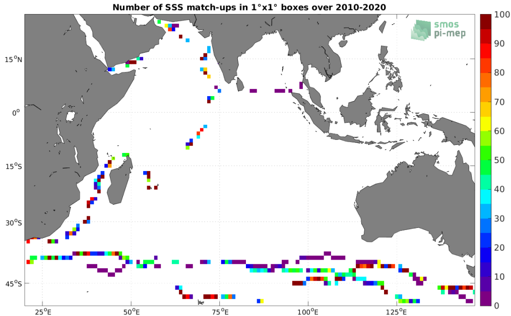
Figure 4: Number of SSS match-ups between TSG (GOSUD-Sailing-ship) SSS and the SMOS SSS L2Q v331 - No FLAG (CMEMS-CATDS-CPDC) SSS product for the Indian Ocean Pi-MEP region over 1^\circ \times 1^\circ boxes and for the full satellite product period.
