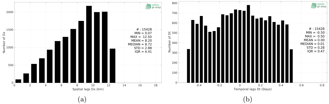
Figure 5: Histograms of the spatial (a) and temporal (b) lags between the location/time of the TSG (GOSUD-Sailing-ship) measurement and the date of the corresponding SMOS SSS L2Q v331 - No FLAG (CMEMS-CATDS-CPDC) SSS pixel.
