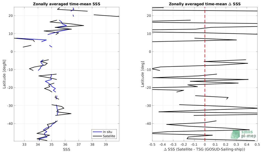
Figure 8: Left panel: Zonal mean SSS from SMOS SSS L2Q v331 - No FLAG (CMEMS-CATDS-CPDC) satellite product (black) and from TSG (GOSUD-Sailing-ship) (blue). Right panel: Zonal mean of \Delta SSS (Satellite - TSG (GOSUD-Sailing-ship)) for all the collected Pi-MEP match-up pairs estimated over the full satellite product period.
