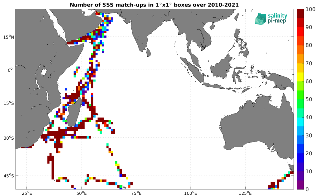
Figure 5: Number of SSS match-ups between TSG (GOSUD-Research-vessel) SSS and the SMOS SSS L2Q v331 - No FLAG (CMEMS-CATDS-CPDC) SSS product for the Indian Ocean Pi-MEP region over 1^\circ \times 1^\circ boxes and for the full satellite product period.
