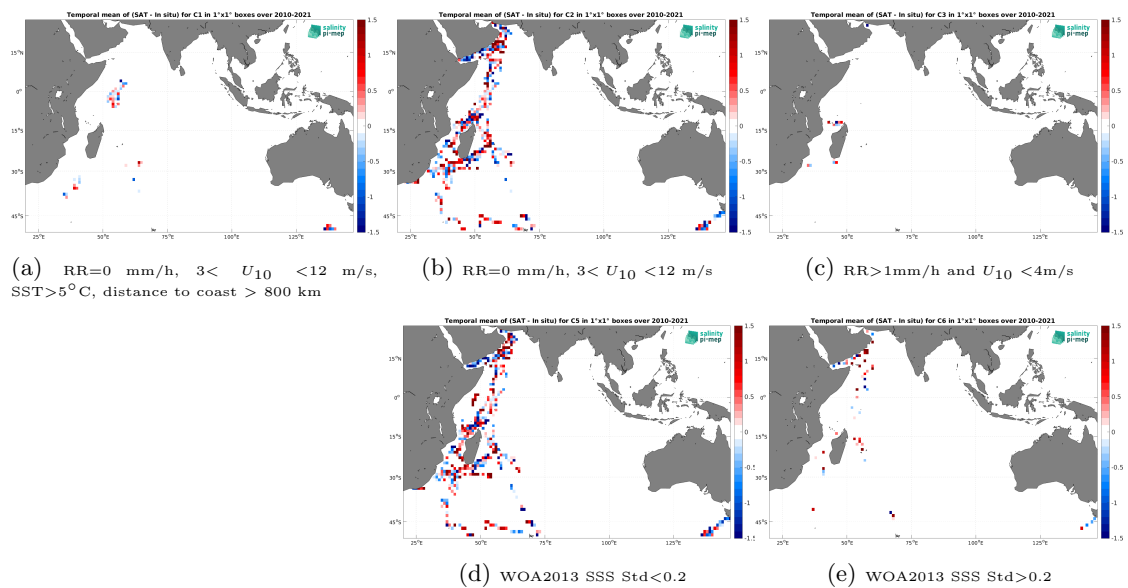
Figure 14: Temporal mean gridded over spatial boxes of size 1^\circ \times 1^\circ of \Delta SSS (SMOS SSS L2Q v331 - No FLAG (CMEMS-CATDS-CPDC) - TSG (GOSUD-Research-vessel)) for 5 different subdatasets corresponding to:RR=0 mm/h, 3 < U_{10} < 12 m/s, SST > 5^\circ\text{C} , distance to coast > 800 km (a), RR=0 mm/h, 3 < U_{10} < 12 m/s (b), RR > 1 mm/h and U_{10} < 4 m/s (c), WOA2013 SSS Std < 0.2 (d), WOA2013 SSS Std > 0.2 (e).
