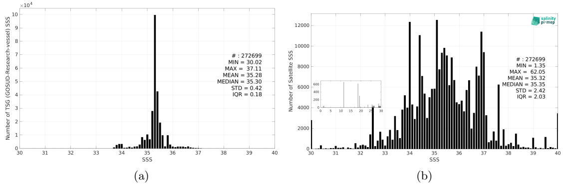
Figure 3: Histograms of SSS from TSG (GOSUD-Research-vessel) (a) and SMOS SSS L2Q v331 - No FLAG (CMEMS-CATDS-CPDC) (b) considering all match-up pairs per bins of 0.1 over the Indian Ocean Pi-MEP region and for the full satellite product period.
