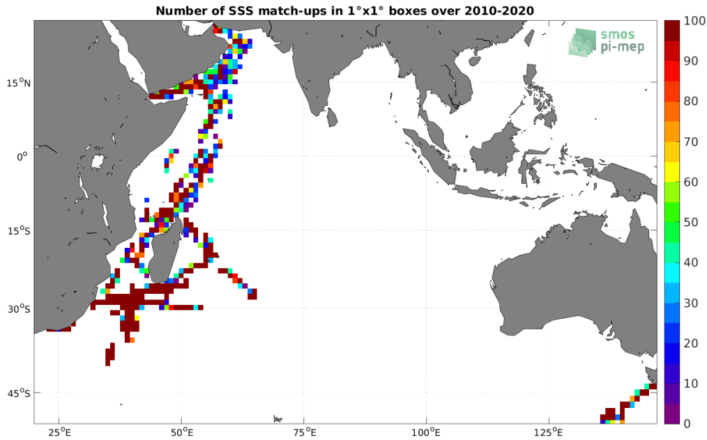
Figure 4: Number of SSS match-ups between TSG (GOSUD-Research-vessel) SSS and the SMOS SSS L2Q v331 - No FLAG (CMEMS-CATDS-CPDC) SSS product for the Indian Ocean Pi-MEP region over 1^\circ \times 1^\circ boxes and for the full satellite product period.
