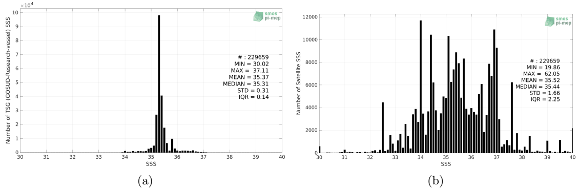
Figure 2: Histograms of SSS from TSG (GOSUD-Research-vessel) (a) and SMOS SSS L2Q v331 - No FLAG (CMEMS-CATDS-CPDC) (b) considering all match-up pairs per bins of 0.1 over the Indian Ocean Pi-MEP region and for the full satellite product period.
