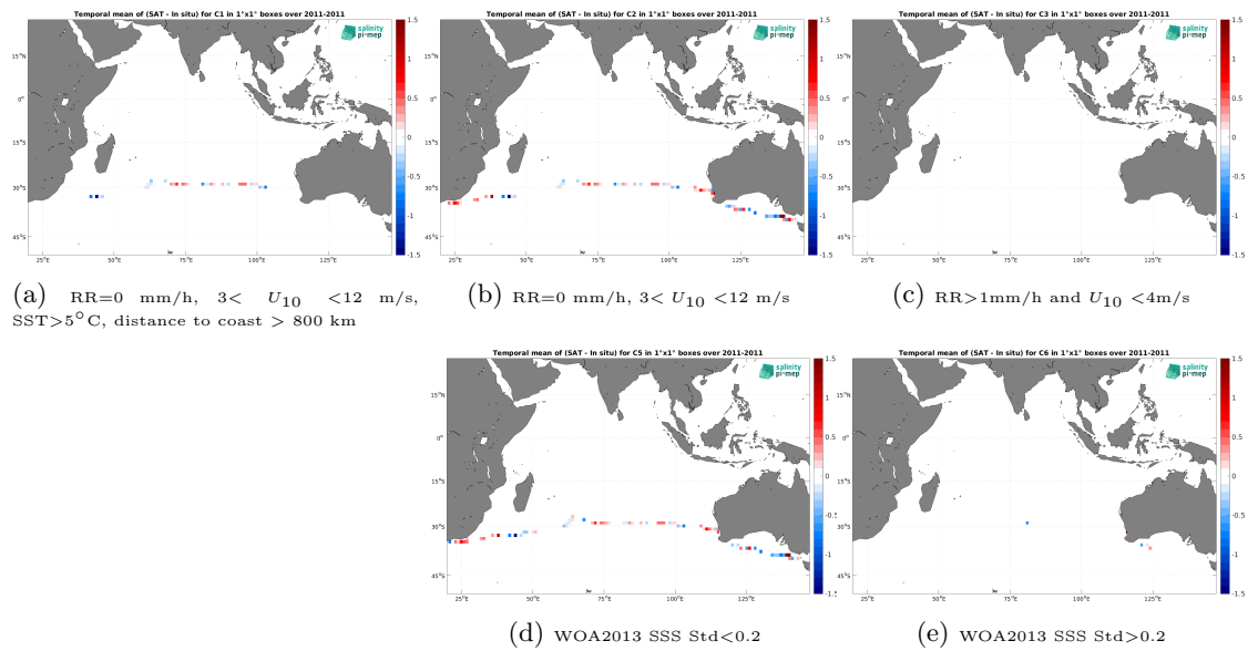
Figure 14: Temporal mean gridded over spatial boxes of size 1^\circ \times 1^\circ of \Delta SSS (SMOS SSS L2Q v331 - No FLAG (CMEMS-CATDS-CPDC) - TSG (CSIC-UTM)) for 5 different subdatasets corresponding to:RR=0 mm/h, 3 < U_{10} < 12 m/s, SST >5^\circ\text{C} , distance to coast > 800 km (a), RR=0 mm/h, 3 < U_{10} < 12 m/s (b), RR >1 mm/h and U_{10} < 4 m/s (c), WOA2013 SSS Std <0.2 (d), WOA2013 SSS Std >0.2 (e).
