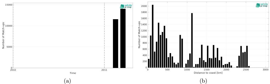
Figure 2: Number of match-ups between TSG (CSIC-UTM) and SMOS SSS L2Q v331 - No FLAG (CMEMS-CATDS-CPDC) SSS as a function of time (a) and as function of the distance to coast (b) over the Indian Ocean Pi-MEP region and for the full satellite product period.
