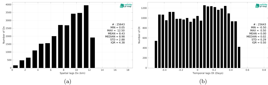
Figure 6: Histograms of the spatial (a) and temporal (b) lags between the location/time of the TSG (CSIC-UTM) measurement and the date of the corresponding SMOS SSS L2Q v331 - No FLAG (CMEMS-CATDS-CPDC) SSS pixel.
