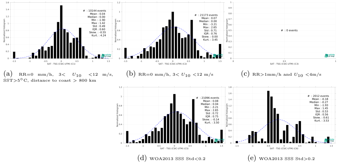
Figure 15: Normalized histogram of \Delta SSS (SMOS SSS L2Q v331 - No FLAG (CMEMS-CATDS-CPDC) - TSG (CSIC-UTM)) for 5 different subdatasets corresponding to: RR=0 mm/h, 3 < U_{10} < 12 m/s, SST > 5°C, distance to coast > 800 km (a), RR=0 mm/h, 3 < U_{10} < 12 m/s (b), RR > 1mm/h and U_{10} < 4 m/s (c), WOA2013 SSS Std < 0.2 (d), WOA2013 SSS Std > 0.2 (e).
