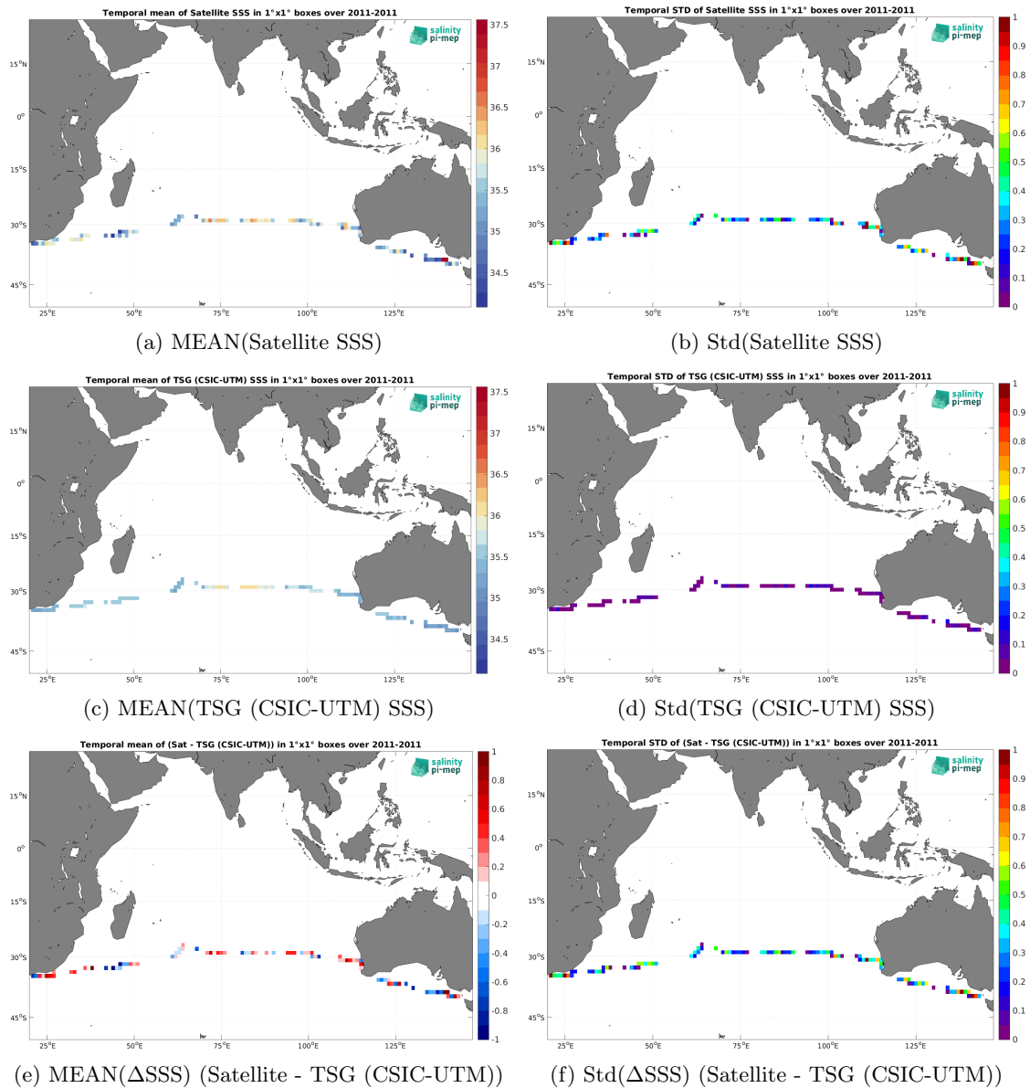
Figure 7: Temporal mean (left) and Std (right) of SSS from SMOS SSS L2Q v331 - No FLAG (CMEMS-CATDS-CPDC) (top), TSG (CSIC-UTM) (middle), and of \Delta SSS (Satellite - TSG (CSIC-UTM)). Only match-up pairs are used to generate these maps.
