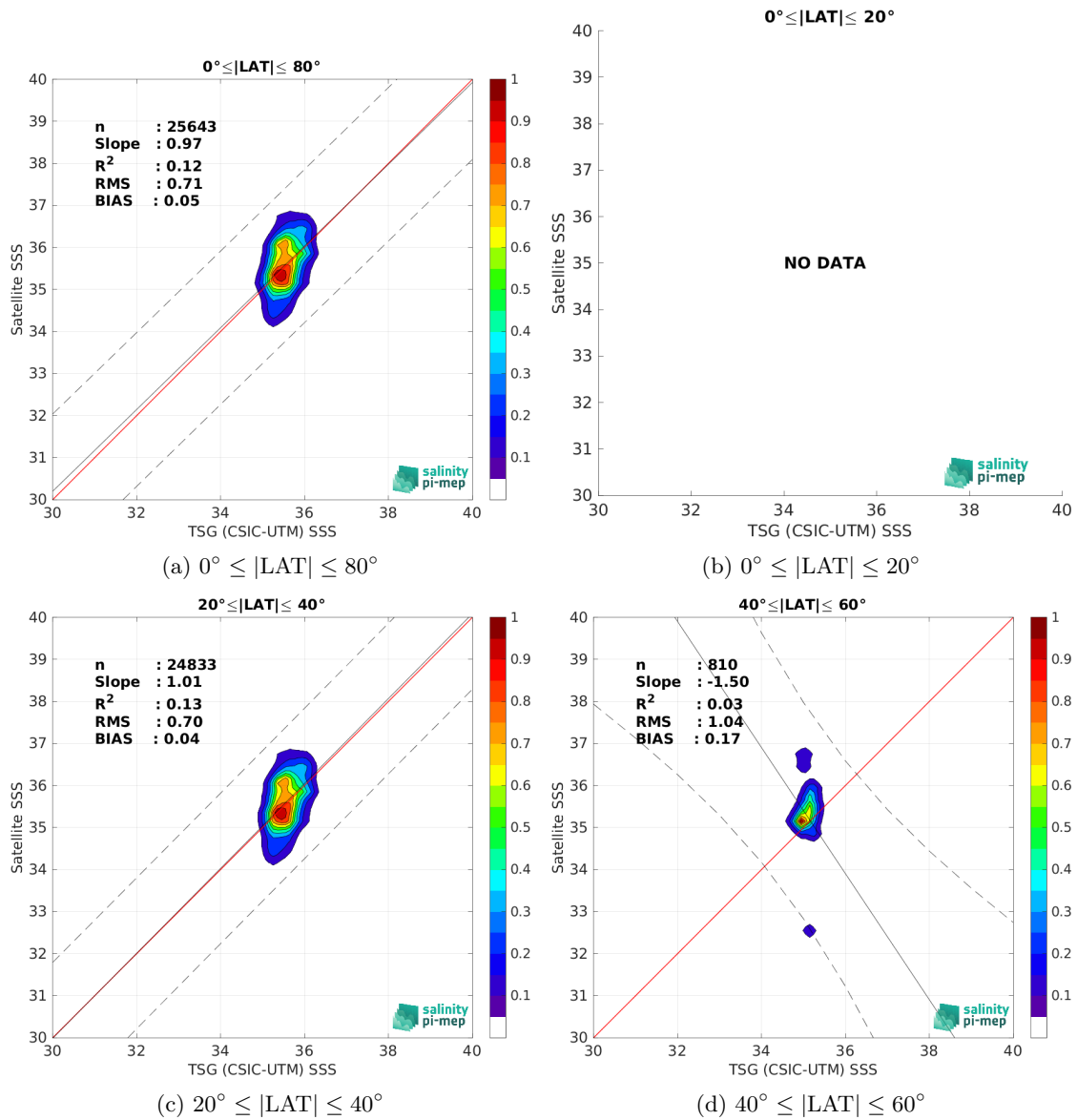
Figure 10: Contour maps of the concentration of SMOS SSS L2Q v331 - No FLAG (CMEMS-CATDS-CPDC) SSS (y-axis) versus TSG (CSIC-UTM) SSS (x-axis) at match-up pairs for different latitude bands. For each plot, the red line shows x=y . The black thin and dashed lines indicate a linear fit through the data cloud and the \pm 95\% confidence levels, respectively. The number match-up pairs n , the slope and R^2 coefficient of the linear fit, the root mean square (RMS) and the mean bias between satellite and in situ data are indicated for each latitude band in each plots.
