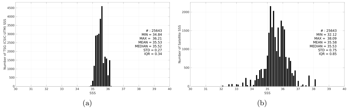
Figure 3: Histograms of SSS from TSG (CSIC-UTM) (a) and SMOS SSS L2Q v331 - No FLAG (CMEMS-CATDS-CPDC) (b) considering all match-up pairs per bins of 0.1 over the Indian Ocean Pi-MEP region and for the full satellite product period.
