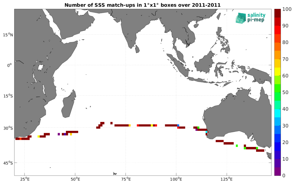
Figure 4: Number of SSS match-ups between TSG (CSIC-UTM) SSS and the SMOS SSS L2Q v331 - No FLAG (CMEMS-CATDS-CPDC) SSS product for the Indian Ocean Pi-MEP region over 1^\circ \times 1^\circ boxes and for the full satellite product period.
