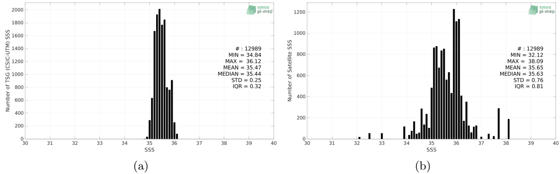
Figure 2: Histograms of SSS from TSG (CSIC-UTM) (a) and SMOS SSS L2Q v331 - No FLAG (CMEMS-CATDS-CPDC) (b) considering all match-up pairs per bins of 0.1 over the Indian Ocean Pi-MEP region and for the full satellite product period.
