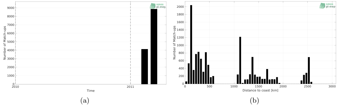
Figure 1: Number of match-ups between TSG (CSIC-UTM) and SMOS SSS L2Q v331 - No FLAG (CMEMS-CATDS-CPDC) SSS as a function of time (a) and as function of the distance to coast (b) over the Indian Ocean Pi-MEP region and for the full satellite product period.
