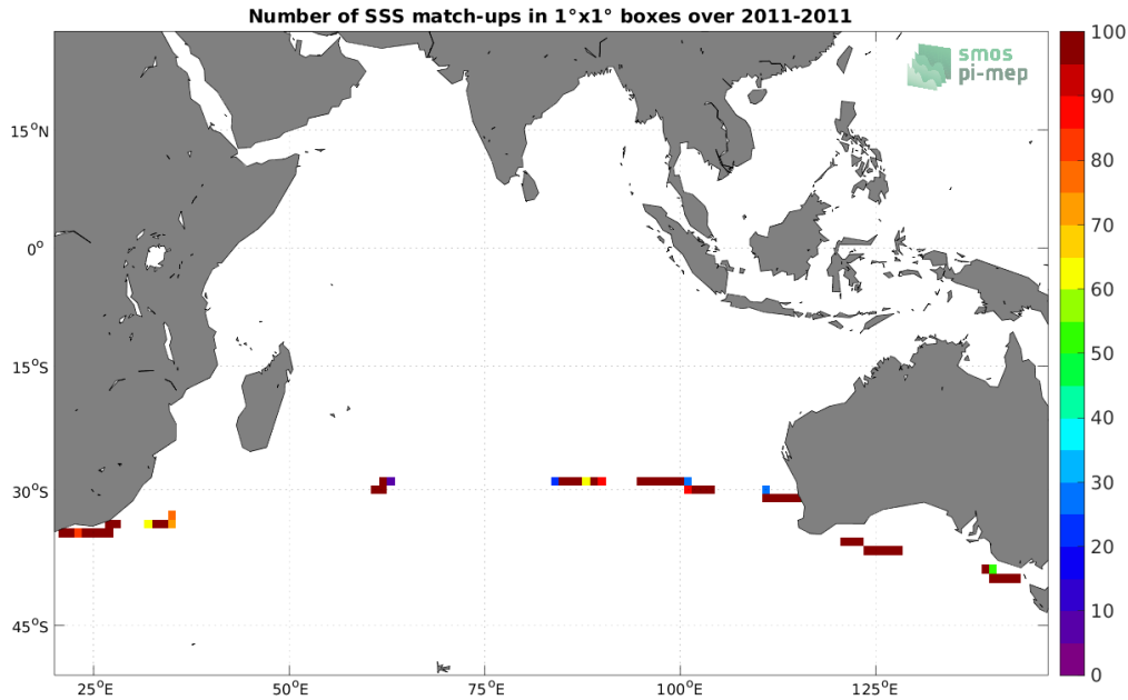
Figure 4: Number of SSS match-ups between TSG (CSIC-UTM) SSS and the SMOS SSS L2Q v331 - No FLAG (CMEMS-CATDS-CPDC) SSS product for the Indian Ocean Pi-MEP region over 1^\circ \times 1^\circ boxes and for the full satellite product period.
