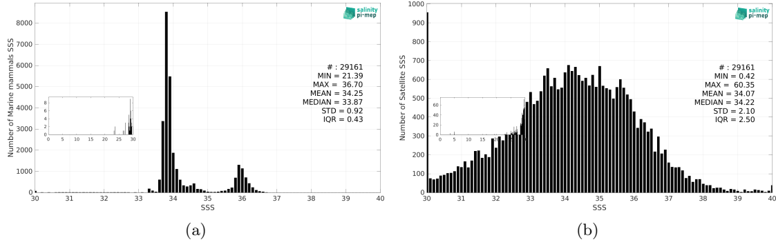
Figure 3: Histograms of SSS from Marine mammals (a) and SMOS SSS L2Q v331 - No FLAG (CMEMS-CATDS-CPDC) (b) considering all match-up pairs per bins of 0.1 over the Indian Ocean Pi-MEP region and for the full satellite product period.
