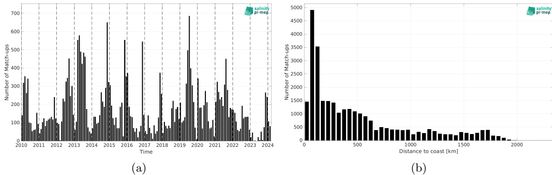
Figure 2: Number of match-ups between Marine mammals and SMOS SSS L2Q v331 - No FLAG (CMEMS-CATDS-CPDC) SSS as a function of time (a) and as function of the distance to coast (b) over the Indian Ocean Pi-MEP region and for the full satellite product period.
