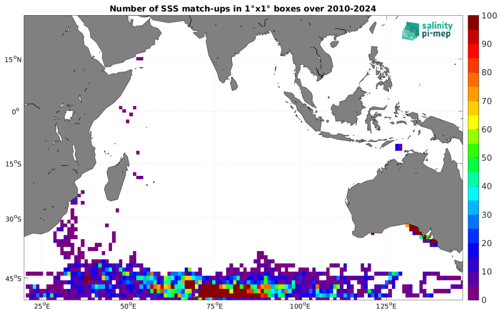
Figure 5: Number of SSS match-ups between Marine mammals SSS and the SMOS SSS L2Q v331 - No FLAG (CMEMS-CATDS-CPDC) SSS product for the Indian Ocean Pi-MEP region over 1^{\circ} \times 1^{\circ} boxes and for the full satellite product period.
