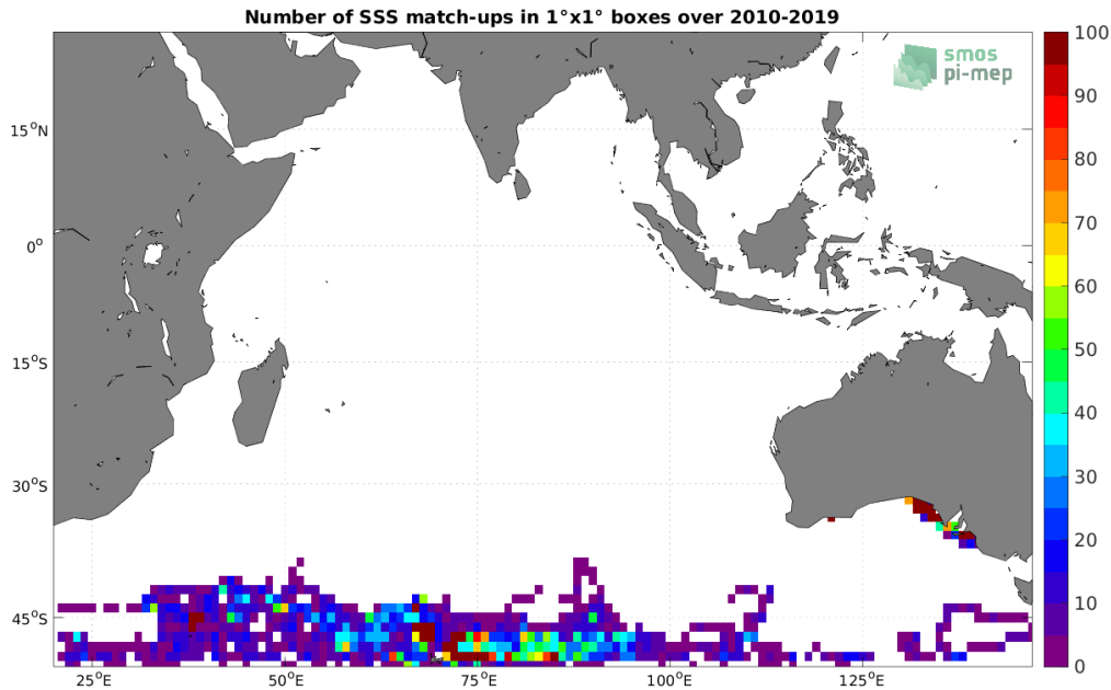
Figure 4: Number of SSS match-ups between Marine mammals SSS and the SMOS SSS L2Q v331 - No FLAG (CMEMS-CATDS-CPDC) SSS product for the Indian Ocean Pi-MEP region over 1^\circ \times 1^\circ boxes and for the full satellite product period.
