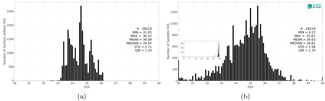
Figure 3: Histograms of SSS from Surface drifters (a) and SMOS SSS L2Q v331 - No FLAG (CMEMS-CATDS-CPDC) (b) considering all match-up pairs per bins of 0.1 over the Indian Ocean Pi-MEP region and for the full satellite product period.
