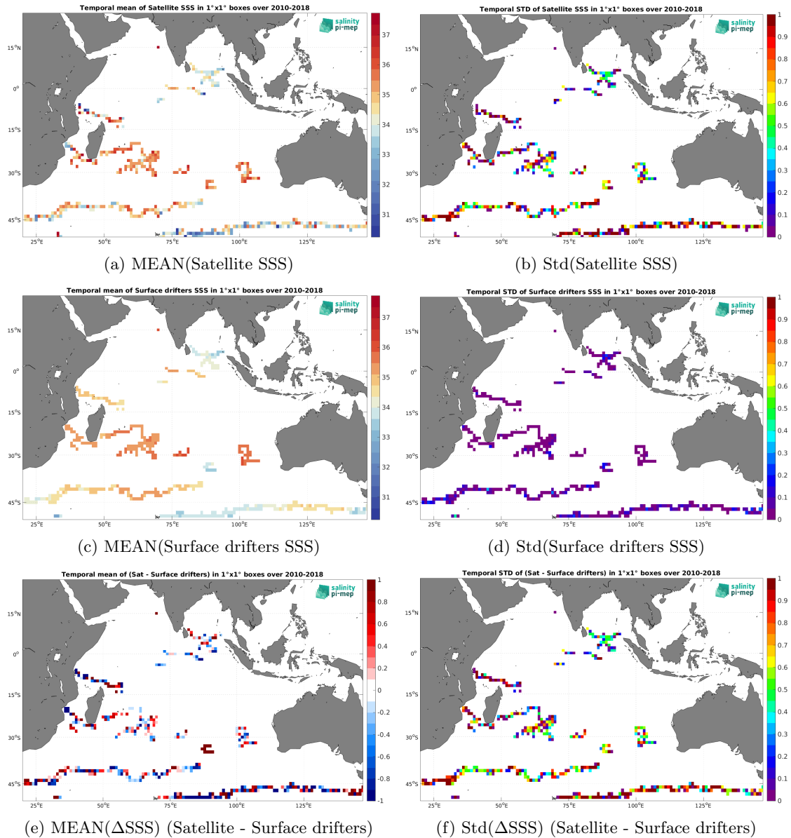
Figure 6: Temporal mean (left) and Std (right) of SSS from SMOS SSS L2Q v331 - No FLAG (CMEMS-CATDS-CPDC) (top), Surface drifters (middle), and of \Delta SSS (Satellite - Surface drifters). Only match-up pairs are used to generate these maps.
