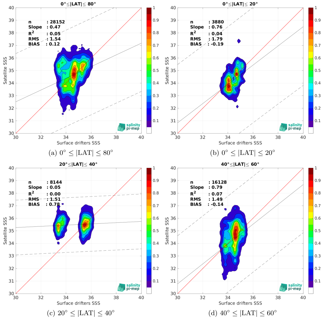
Figure 9: Contour maps of the concentration of SMOS SSS L2Q v331 - No FLAG (CMEMS-CATDS-CPDC) SSS (y-axis) versus Surface drifters SSS (x-axis) at match-up pairs for different latitude bands. For each plot, the red line shows x=y . The black thin and dashed lines indicate a linear fit through the data cloud and the \pm 95\% confidence levels, respectively. The number match-up pairs n , the slope and R^2 coefficient of the linear fit, the root mean square (RMS) and the mean bias between satellite and in situ data are indicated for each latitude band in each plots.
