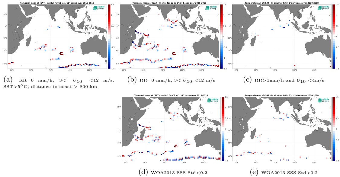
Figure 13: Temporal mean gridded over spatial boxes of size 1^\circ \times 1^\circ of \Delta SSS (SMOS SSS L2Q v331 - No FLAG (CMEMS-CATDS-CPDC) - Surface drifters) for 5 different subdatasets corresponding to:RR=0 mm/h, 3 < U_{10} < 12 m/s, SST >5^\circ C, distance to coast > 800 km (a), RR=0 mm/h, 3 < U_{10} < 12 m/s (b), RR >1 mm/h and U_{10} < 4 m/s (c), WOA2013 SSS Std <0.2 (d), WOA2013 SSS Std >0.2 (e).
