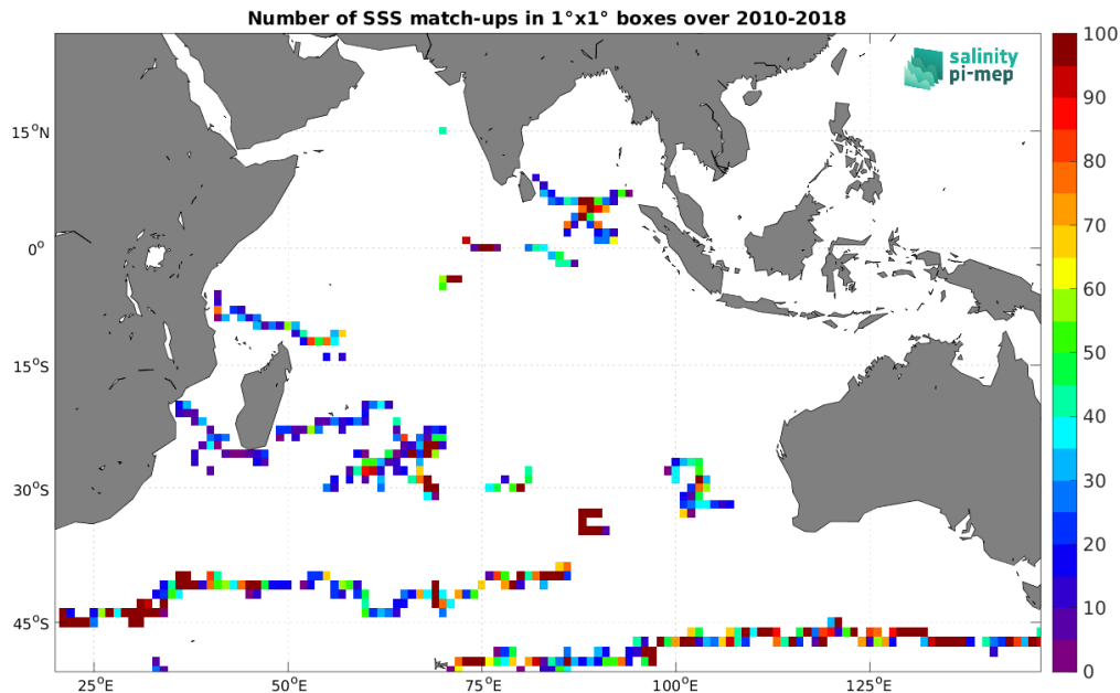
Figure 4: Number of SSS match-ups between Surface drifters SSS and the SMOS SSS L2Q v331 - No FLAG (CMEMS-CATDS-CPDC) SSS product for the Indian Ocean Pi-MEP region over 1^\circ \times 1^\circ boxes and for the full satellite product period.
