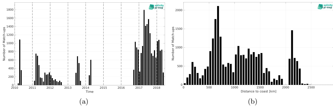
Figure 2: Number of match-ups between Surface drifters and SMOS SSS L2Q v331 - No FLAG (CMEMS-CATDS-CPDC) SSS as a function of time (a) and as function of the distance to coast (b) over the Indian Ocean Pi-MEP region and for the full satellite product period.
