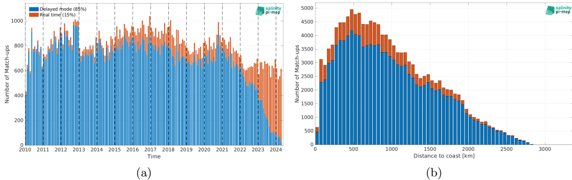
Figure 2: Number of match-ups between Argo and SMOS SSS L2Q v331 - No FLAG (CMEMS-CATDS-CPDC) SSS as a function of time (a) and as function of the distance to coast (b) over the Indian Ocean Pi-MEP region and for the full satellite product period.
