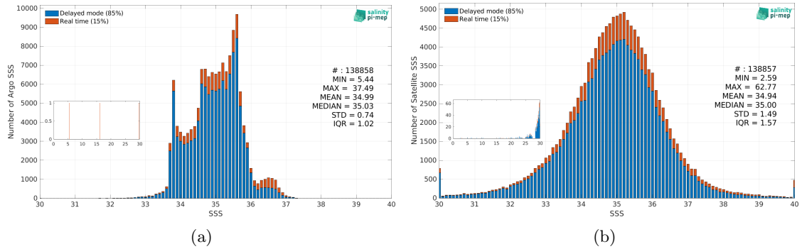
Figure 3: Histograms of SSS from Argo (a) and SMOS SSS L2Q v331 - No FLAG (CMEMS-CATDS-CPDC) (b) considering all match-up pairs per bins of 0.1 over the Indian Ocean Pi-MEP region and for the full satellite product period.
