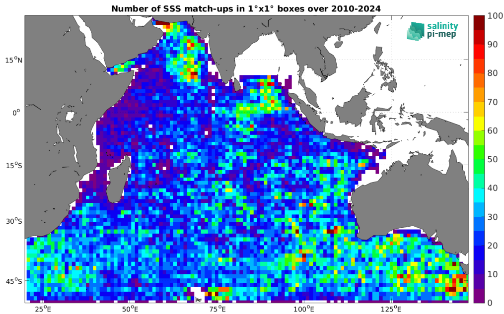
Figure 5: Number of SSS match-ups between Argo SSS and the SMOS SSS L2Q v331 - No FLAG (CMEMS-CATDS-CPDC) SSS product for the Indian Ocean Pi-MEP region over 1^\circ \times 1^\circ boxes and for the full satellite product period.
