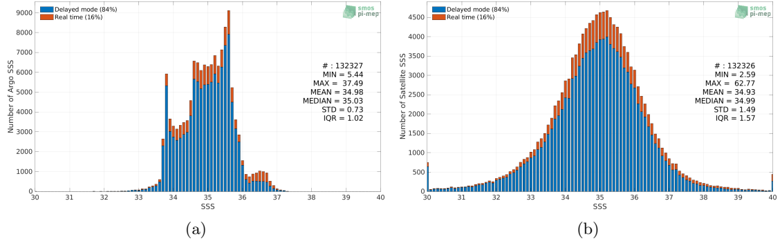
Figure 2: Histograms of SSS from Argo (a) and SMOS SSS L2Q v331 - No FLAG (CMEMS-CATDS-CPDC) (b) considering all match-up pairs per bins of 0.1 over the Indian Ocean Pi-MEP region and for the full satellite product period.
