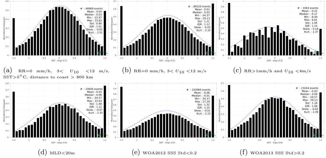
Figure 13: Normalized histogram of \Delta SSS (SMOS SSS L2Q v331 - No FLAG (CMEMS-CATDS-CPDC) - Argo) for 6 different subdatasets corresponding to: RR=0 mm/h, 3 < U_{10} < 12 m/s, SST>5°C, distance to coast > 800 km (a), RR=0 mm/h, 3 < U_{10} < 12 m/s (b), RR>1mm/h and U_{10} < 4 m/s (c), MLD<20m (d), WOA2013 SSS Std<0.2 (e), WOA2013 SSS Std>0.2 (f).
