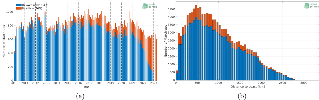
Figure 1: Number of match-ups between Argo and SMOS SSS L2Q v331 - No FLAG (CMEMS-CATDS-CPDC) SSS as a function of time (a) and as function of the distance to coast (b) over the Indian Ocean Pi-MEP region and for the full satellite product period.
