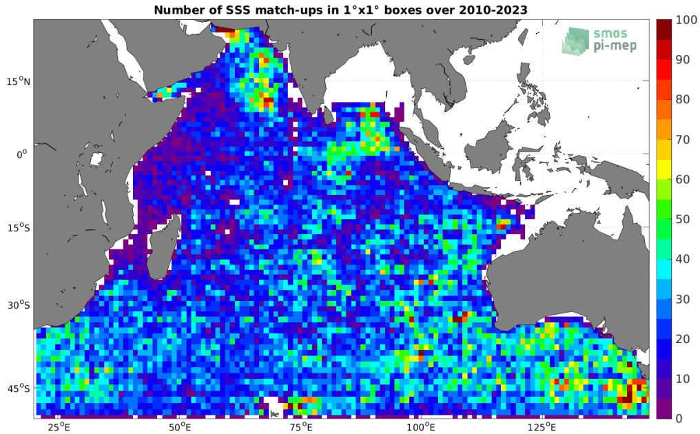
Figure 4: Number of SSS match-ups between Argo SSS and the SMOS SSS L2Q v331 - No FLAG (CMEMS-CATDS-CPDC) SSS product for the Indian Ocean Pi-MEP region over 1^\circ \times 1^\circ boxes and for the full satellite product period.
