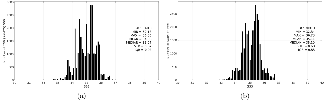
Figure 3: Histograms of SSS from TSG (SAMOS) (a) and SMOS SSS L3 v9 - 9 Days (CATDS-CEC-LOCEAN) (b) considering all match-up pairs per bins of 0.1 over the Indian Ocean Pi-MEP region and for the full satellite product period.
