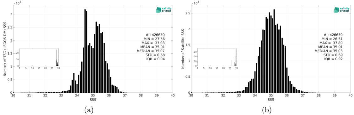
Figure 3: Histograms of SSS from TSG (LEGOS-DM) (a) and SMOS SSS L3 v9 - 9 Days (CATDS-CEC-LOCEAN) (b) considering all match-up pairs per bins of 0.1 over the Indian Ocean Pi-MEP region and for the full satellite product period.
