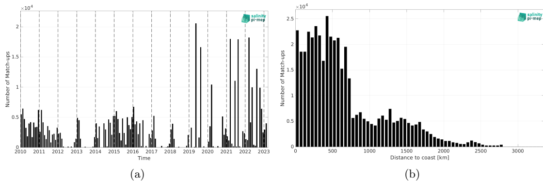
Figure 2: Number of match-ups between TSG (LEGOS-DM) and SMOS SSS L3 v9 - 9 Days (CATDS-CEC-LOCEAN) SSS as a function of time (a) and as function of the distance to coast (b) over the Indian Ocean Pi-MEP region and for the full satellite product period.
