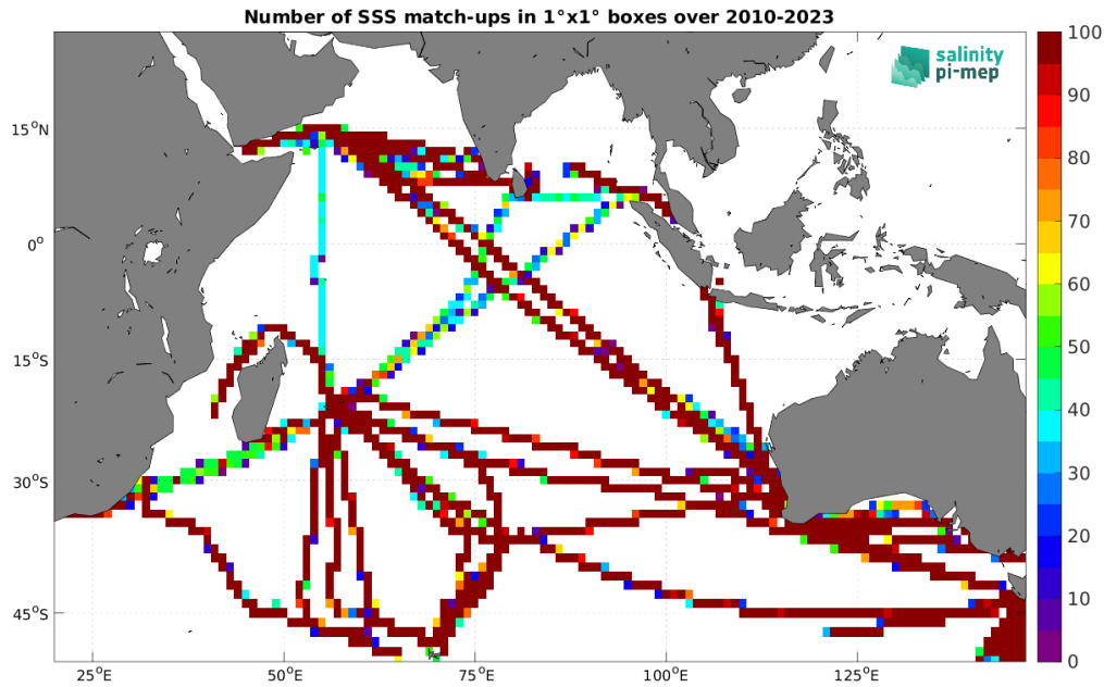
Figure 5: Number of SSS match-ups between TSG (LEGOS-DM) SSS and the SMOS SSS L3 v9 - 9 Days (CATDS-CEC-LOCEAN) SSS product for the Indian Ocean Pi-MEP region over 1^\circ \times 1^\circ boxes and for the full satellite product period.
