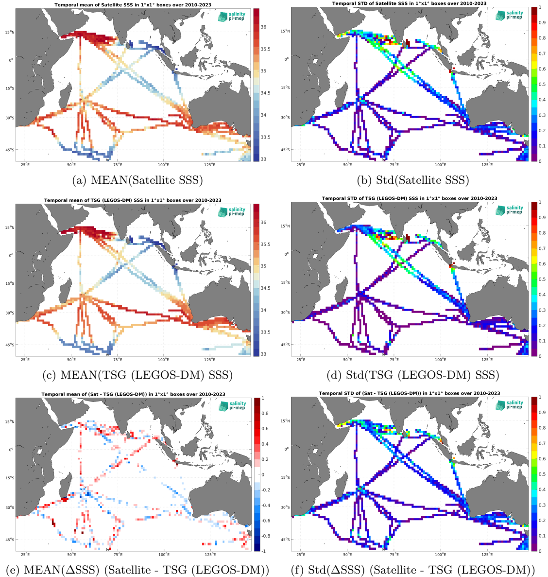
Figure 6: Temporal mean (left) and Std (right) of SSS from SMOS SSS L3 v9 - 9 Days (CATDS-CEC-LOCEAN) (top), TSG (LEGOS-DM) (middle), and of \Delta SSS (Satellite - TSG (LEGOS-DM)). Only match-up pairs are used to generate these maps.
