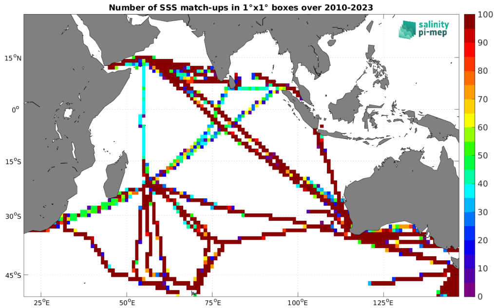
Figure 4: Number of SSS match-ups between TSG (LEGOS-DM) SSS and the SMOS SSS L3 v9 - 9 Days (CATDS-CEC-LOCEAN) SSS product for the Indian Ocean Pi-MEP region over 1^\circ \times 1^\circ boxes and for the full satellite product period.
