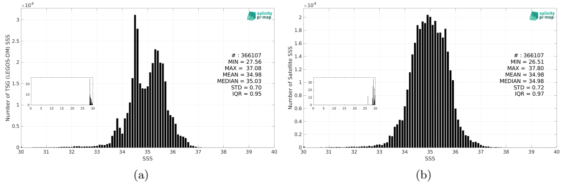
Figure 2: Histograms of SSS from TSG (LEGOS-DM) (a) and SMOS SSS L3 v9 - 9 Days (CATDS-CEC-LOCEAN) (b) considering all match-up pairs per bins of 0.1 over the Indian Ocean Pi-MEP region and for the full satellite product period.
