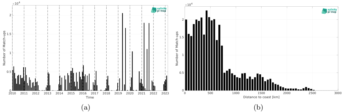
Figure 1: Number of match-ups between TSG (LEGOS-DM) and SMOS SSS L3 v9 - 9 Days (CATDS-CEC-LOCEAN) SSS as a function of time (a) and as function of the distance to coast (b) over the Indian Ocean Pi-MEP region and for the full satellite product period.
