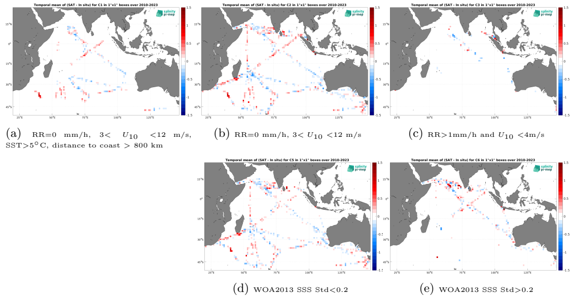
Figure 12: Temporal mean gridded over spatial boxes of size 1^\circ \times 1^\circ of \Delta SSS (SMOS SSS L3 v9 - 9 Days (CATDS-CEC-LOCEAN) - TSG (LEGOS-DM)) for 5 different subdatasets corresponding to:RR=0 mm/h, 3 < U_{10} < 12 m/s, SST >5^\circ C, distance to coast > 800 km (a), RR=0 mm/h, 3 < U_{10} < 12 m/s (b), RR >1 mm/h and U_{10} < 4 m/s (c), WOA2013 SSS Std <0.2 (d), WOA2013 SSS Std >0.2 (e).
