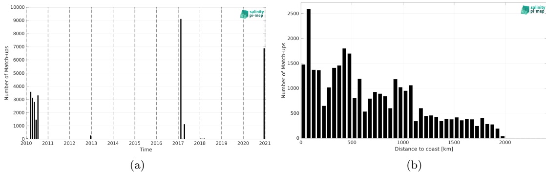
Figure 2: Number of match-ups between TSG (GOSUD-Sailing-ship) and SMOS SSS L3 v9 - 9 Days (CATDS-CEC-LOCEAN) SSS as a function of time (a) and as function of the distance to coast (b) over the Indian Ocean Pi-MEP region and for the full satellite product period.
