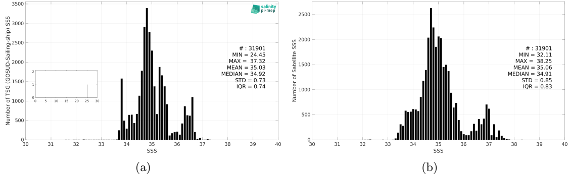
Figure 3: Histograms of SSS from TSG (GOSUD-Sailing-ship) (a) and SMOS SSS L3 v9 - 9 Days (CATDS-CEC-LOCEAN) (b) considering all match-up pairs per bins of 0.1 over the Indian Ocean Pi-MEP region and for the full satellite product period.
