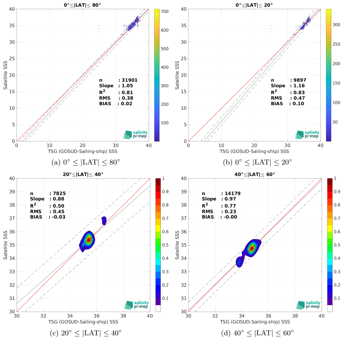
Figure 10: Contour maps of the concentration of SMOS SSS L3 v9 - 9 Days (CATDS-CEC-LOCEAN) SSS ( y -axis) versus TSG (GOSUD-Sailing-ship) SSS ( x -axis) at match-up pairs for different latitude bands. For each plot, the red line shows x=y . The black thin and dashed lines indicate a linear fit through the data cloud and the \pm 95\% confidence levels, respectively. The number match-up pairs n , the slope and R^2 coefficient of the linear fit, the root mean square (RMS) and the mean bias between satellite and in situ data are indicated for each latitude band in each plots.
