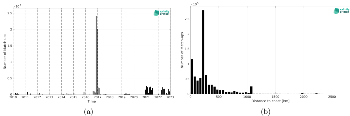
Figure 2: Number of match-ups between TSG (GOSUD-Research-vessel) and SMOS SSS L3 v9 - 9 Days (CATDS-CEC-LOCEAN) SSS as a function of time (a) and as function of the distance to coast (b) over the Indian Ocean Pi-MEP region and for the full satellite product period.
