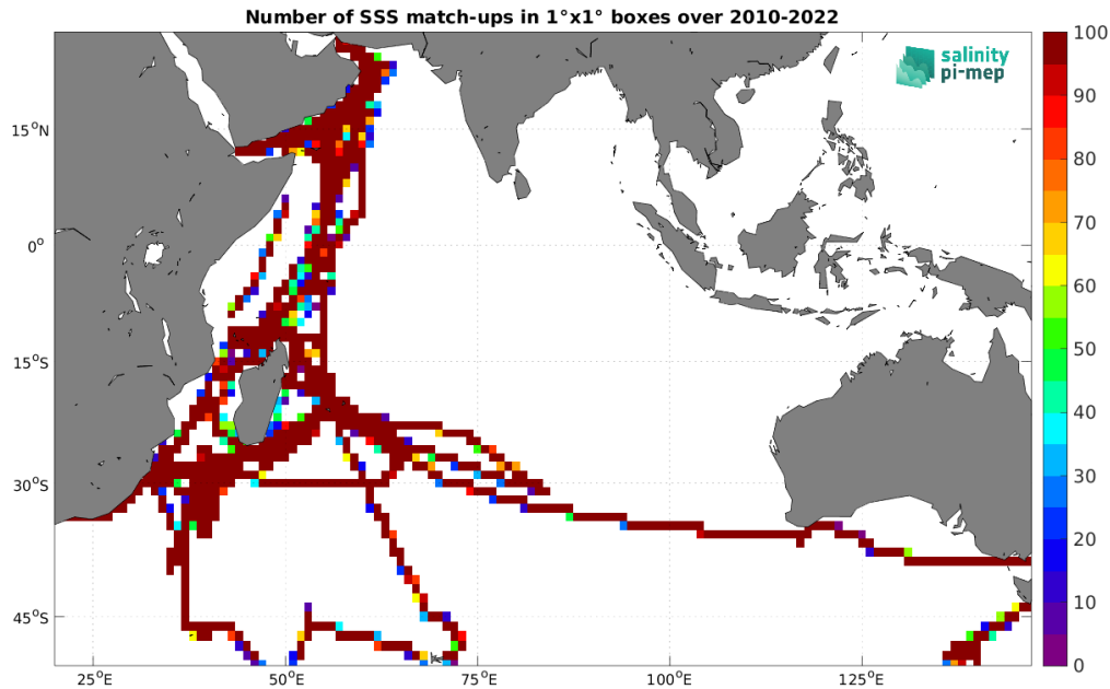
Figure 5: Number of SSS match-ups between TSG (GOSUD-Research-vessel) SSS and the SMOS SSS L3 v9 - 9 Days (CATDS-CEC-LOCEAN) SSS product for the Indian Ocean Pi-MEP region over 1^\circ \times 1^\circ boxes and for the full satellite product period.
