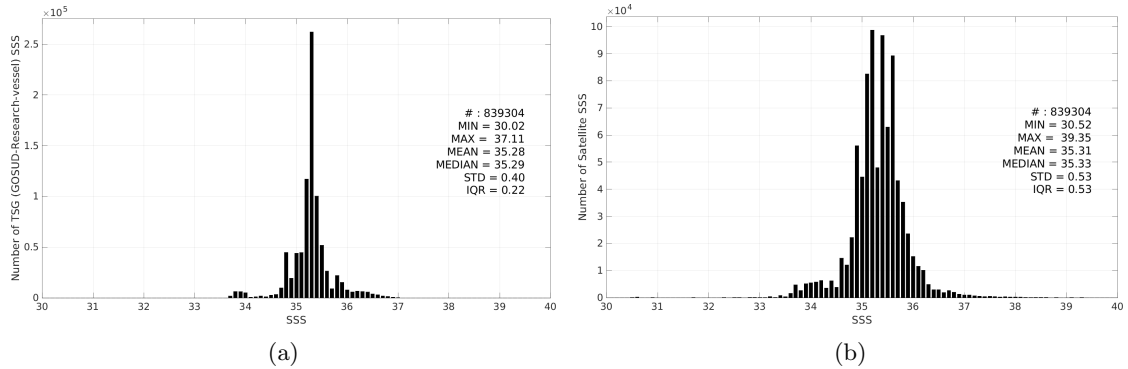
Figure 3: Histograms of SSS from TSG (GOSUD-Research-vessel) (a) and SMOS SSS L3 v9 - 9 Days (CATDS-CEC-LOCEAN) (b) considering all match-up pairs per bins of 0.1 over the Indian Ocean Pi-MEP region and for the full satellite product period.
