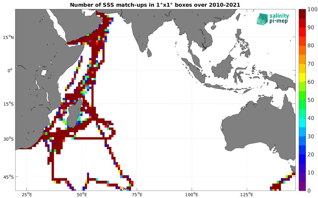
Figure 5: Number of SSS match-ups between TSG (GOSUD-Research-vessel) SSS and the SMOS SSS L3 v9 - 9 Days (CATDS-CEC-LOCEAN) SSS product for the Indian Ocean Pi-MEP region over 1^\circ \times 1^\circ boxes and for the full satellite product period.
