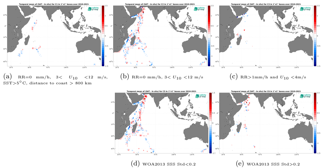
Figure 12: Temporal mean gridded over spatial boxes of size 1^\circ \times 1^\circ of \Delta SSS (SMOS SSS L3 v9 - 9 Days (CATDS-CEC-LOCEAN) - TSG (GOSUD-Research-vessel)) for 5 different subdatasets corresponding to:RR=0 mm/h, 3 < U_{10} < 12 m/s, SST >5^\circ C, distance to coast > 800 km (a), RR=0 mm/h, 3 < U_{10} < 12 m/s (b), RR >1 mm/h and U_{10} < 4 m/s (c), WOA2013 SSS Std <0.2 (d), WOA2013 SSS Std >0.2 (e).
