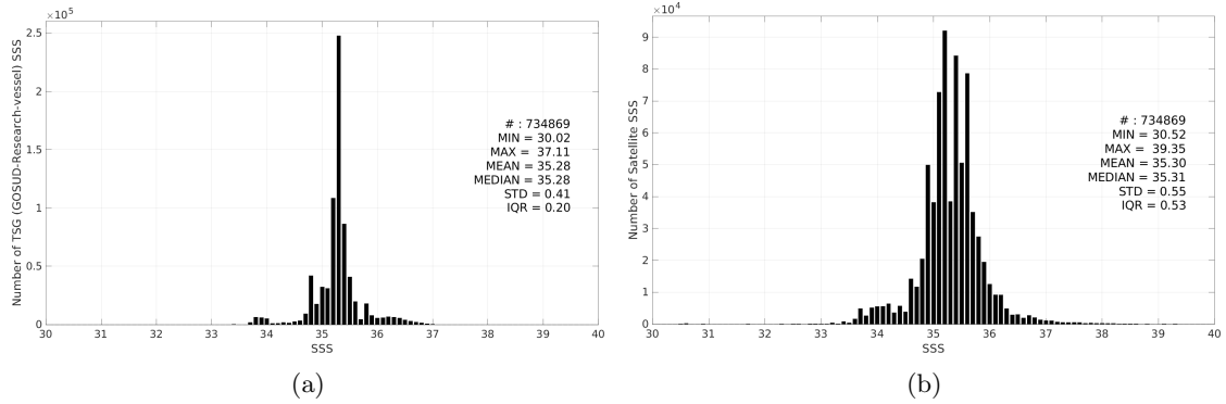
Figure 2: Histograms of SSS from TSG (GOSUD-Research-vessel) (a) and SMOS SSS L3 v9 - 9 Days (CATDS-CEC-LOCEAN) (b) considering all match-up pairs per bins of 0.1 over the Indian Ocean Pi-MEP region and for the full satellite product period.
