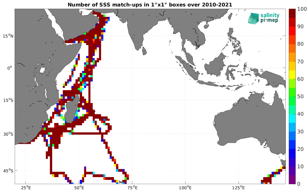
Figure 4: Number of SSS match-ups between TSG (GOSUD-Research-vessel) SSS and the SMOS SSS L3 v9 - 9 Days (CATDS-CEC-LOCEAN) SSS product for the Indian Ocean Pi-MEP region over 1°×1° boxes and for the full satellite product period.
