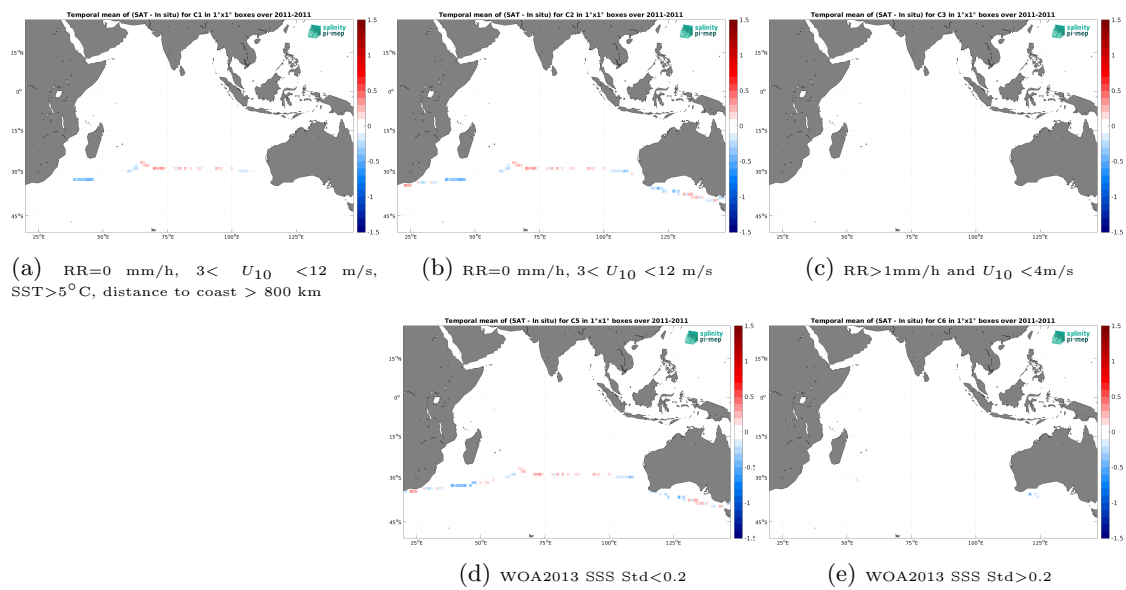
Figure 14: Temporal mean gridded over spatial boxes of size 1^\circ \times 1^\circ of \Delta SSS (SMOS SSS L3 v9 - 9 Days (CATDS-CEC-LOCEAN) - TSG (CSIC-UTM)) for 5 different subdatasets corresponding to: RR=0 mm/h, 3 < U_{10} < 12 m/s, SST > 5^\circ\text{C} , distance to coast > 800 km (a), RR=0 mm/h, 3 < U_{10} < 12 m/s (b), RR > 1\text{mm/h} and U_{10} < 4\text{m/s} (c), WOA2013 SSS Std < 0.2 (d), WOA2013 SSS Std > 0.2 (e).
