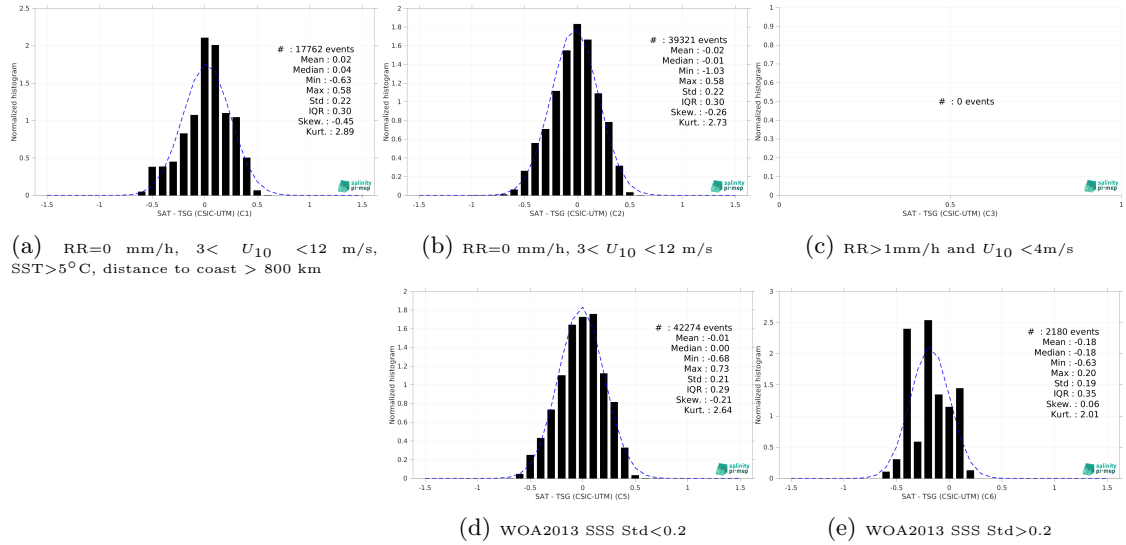
Figure 15: Normalized histogram of \Delta SSS (SMOS SSS L3 v9 - 9 Days (CATDS-CEC-LOCEAN) - TSG (CSIC-UTM)) for 5 different subdatasets corresponding to: RR=0 mm/h, 3 < U_{10} < 12 m/s, SST>5°C, distance to coast > 800 km (a), RR=0 mm/h, 3 < U_{10} < 12 m/s (b), RR>1mm/h and U_{10} < 4 m/s (c), WOA2013 SSS Std<0.2 (d), WOA2013 SSS Std>0.2 (e).
