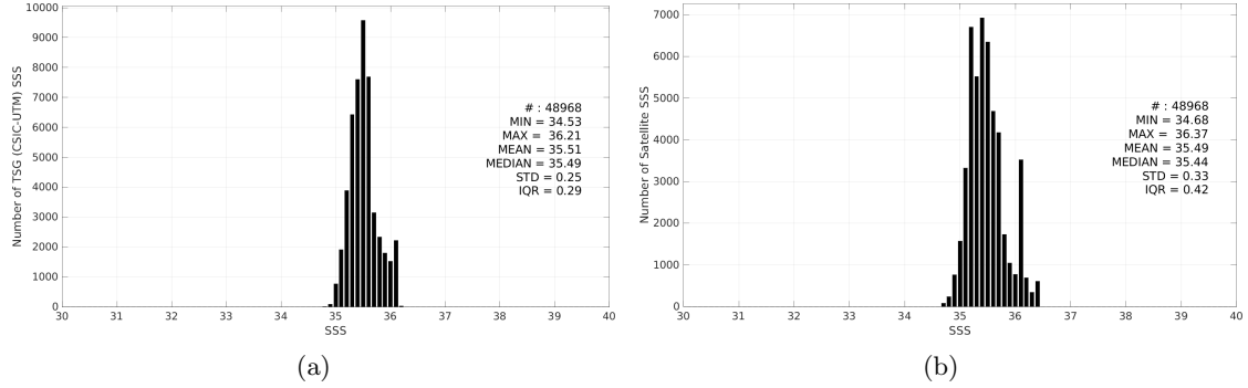
Figure 3: Histograms of SSS from TSG (CSIC-UTM) (a) and SMOS SSS L3 v9 - 9 Days (CATDS-CEC-LOCEAN) (b) considering all match-up pairs per bins of 0.1 over the Indian Ocean Pi-MEP region and for the full satellite product period.
