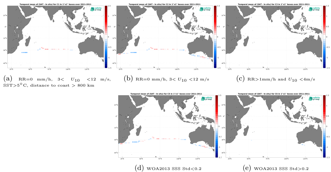
Figure 14: Temporal mean gridded over spatial boxes of size 1^\circ \times 1^\circ of \Delta\text{SSS} (SMOS SSS L3 v9 - 9 Days (CATDS-CEC-LOCEAN) - TSG (CSIC-UTM)) for 5 different subdatasets corresponding to: RR=0 mm/h, 3 < U_{10} < 12 m/s, SST > 5^\circ\text{C} , distance to coast > 800 km (a), RR=0 mm/h, 3 < U_{10} < 12 m/s (b), RR > 1 mm/h and U_{10} < 4 m/s (c), WOA2013 SSS Std < 0.2 (d), WOA2013 SSS Std > 0.2 (e).
