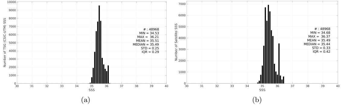
Figure 2: Histograms of SSS from TSG (CSIC-UTM) (a) and SMOS SSS L3 v9 - 9 Days (CATDS-CEC-LOCEAN) (b) considering all match-up pairs per bins of 0.1 over the Indian Ocean Pi-MEP region and for the full satellite product period.
