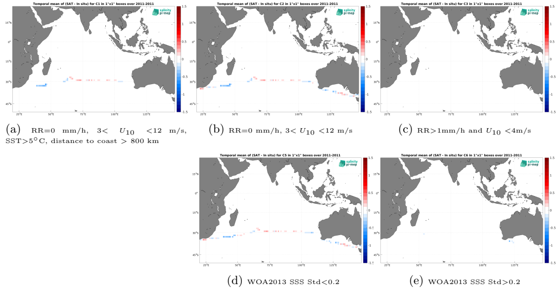
Figure 12: Temporal mean gridded over spatial boxes of size 1^{\circ}\times 1^{\circ} of \Delta\text{SSS} (SMOS SSS L3 v9 - 9 Days (CATDS-CEC-LOCEAN) - TSG (CSIC-UTM)) for 5 different subdatasets corresponding to:RR=0 mm/h, 3 < U_{10} < 12 m/s, SST >5^{\circ}\text{C} , distance to coast > 800 km (a), RR=0 mm/h, 3 < U_{10} < 12 m/s (b), RR >1 mm/h and U_{10} < 4 m/s (c), WOA2013 SSS Std <0.2 (d), WOA2013 SSS Std >0.2 (e).
