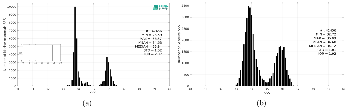
Figure 2: Histograms of SSS from Marine mammals (a) and SMOS SSS L3 v9 - 9 Days (CATDS-CEC-LOCEAN) (b) considering all match-up pairs per bins of 0.1 over the Indian Ocean Pi-MEP region and for the full satellite product period.
