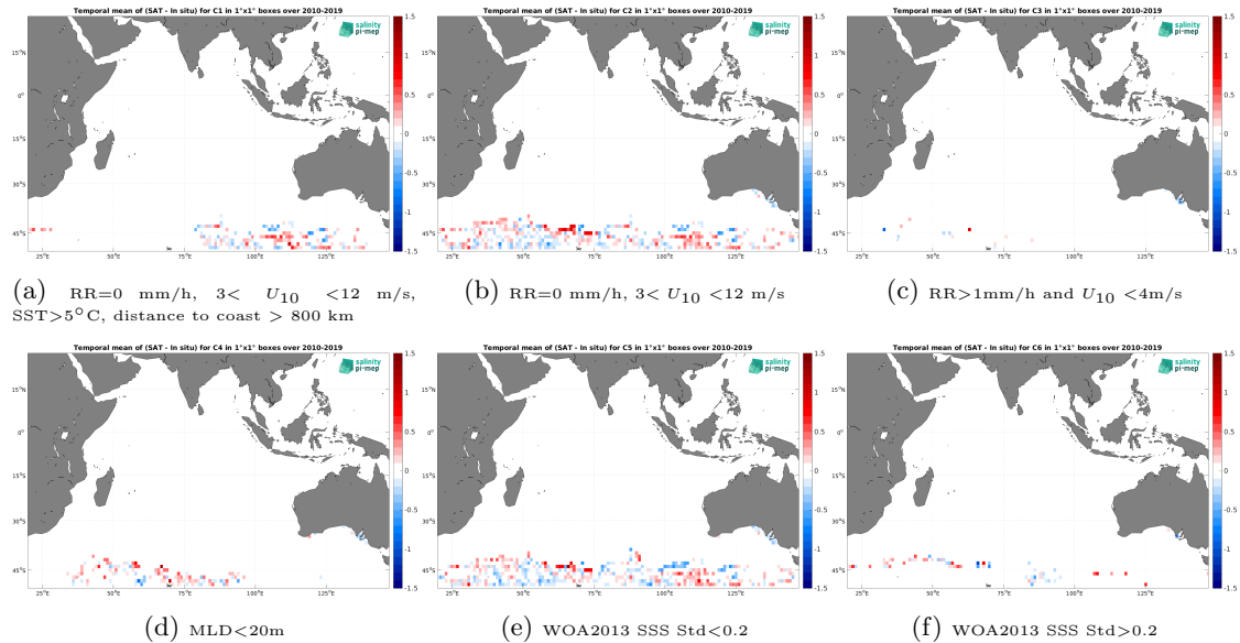
Figure 12: Temporal mean gridded over spatial boxes of size 1^{\circ}\times 1^{\circ} of \Delta\text{SSS} (SMOS SSS L3 v9 - 9 Days (CATDS-CEC-LOCEAN) - Marine mammals) for 6 different subdatasets corresponding to: \text{RR}=0 mm/h, 3 < U_{10} < 12 m/s, \text{SST} > 5^{\circ}\text{C} , distance to coast > 800 km (a), \text{RR}=0 mm/h, 3 < U_{10} < 12 m/s (b), \text{RR} > 1\text{mm/h} and U_{10} < 4\text{m/s} (c), \text{MLD} < 20\text{m} (d), WOA2013 SSS Std < 0.2 (e), WOA2013 SSS Std > 0.2 (f).
