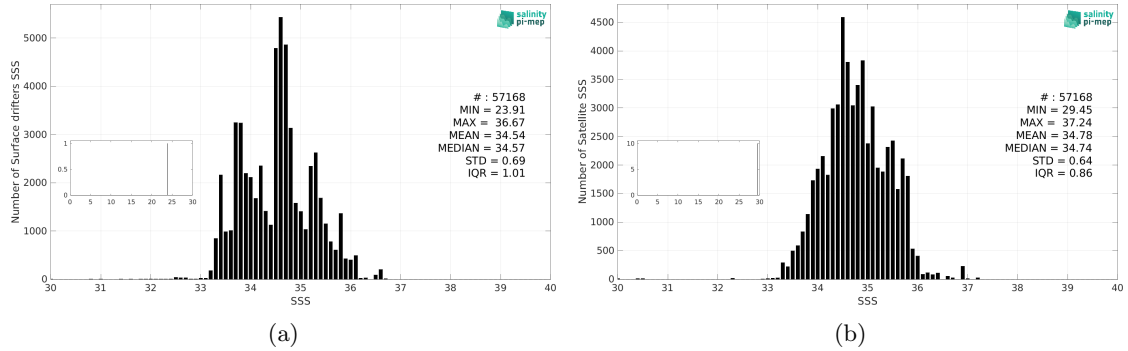
Figure 3: Histograms of SSS from Surface drifters (a) and SMOS SSS L3 v9 - 9 Days (CATDS-CEC-LOCEAN) (b) considering all match-up pairs per bins of 0.1 over the Indian Ocean Pi-MEP region and for the full satellite product period.
