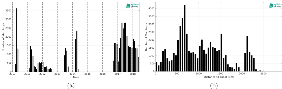
Figure 2: Number of match-ups between Surface drifters and SMOS SSS L3 v9 - 9 Days (CATDS-CEC-LOCEAN) SSS as a function of time (a) and as function of the distance to coast (b) over the Indian Ocean Pi-MEP region and for the full satellite product period.
