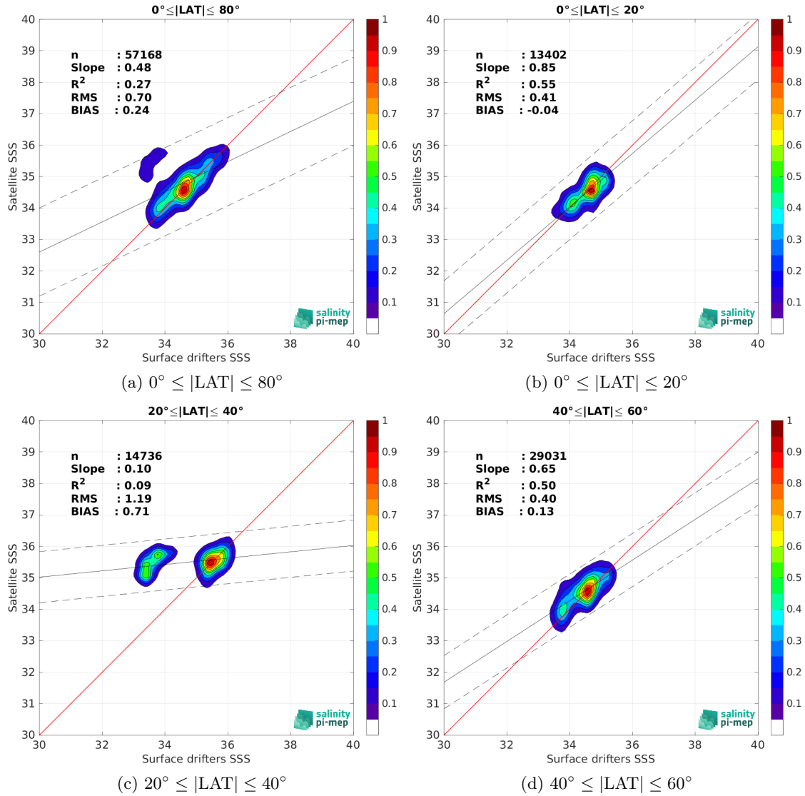
Figure 9: Contour maps of the concentration of SMOS SSS L3 v9 - 9 Days (CATDS-CEC-LOCEAN) SSS ( y -axis) versus Surface drifters SSS ( x -axis) at match-up pairs for different latitude bands. For each plot, the red line shows x=y . The black thin and dashed lines indicate a linear fit through the data cloud and the \pm 95\% confidence levels, respectively. The number match-up pairs n , the slope and R^2 coefficient of the linear fit, the root mean square (RMS) and the mean bias between satellite and in situ data are indicated for each latitude band in each plots.
