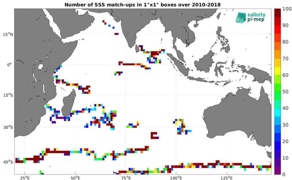
Figure 4: Number of SSS match-ups between Surface drifters SSS and the SMOS SSS L3 v9 - 9 Days (CATDS-CEC-LOCEAN) SSS product for the Indian Ocean Pi-MEP region over 1^\circ \times 1^\circ boxes and for the full satellite product period.
