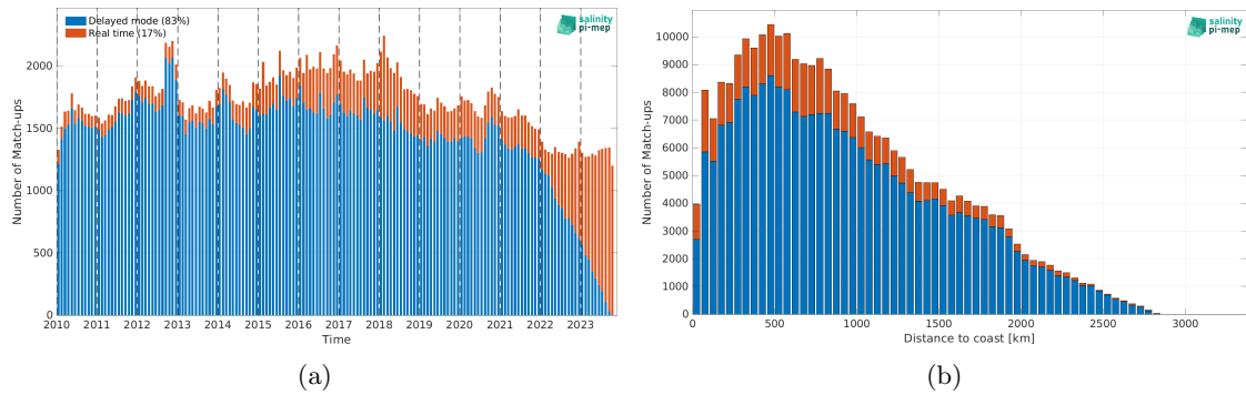
Figure 1: Number of match-ups between Argo and SMOS SSS L3 v9 - 9 Days (CATDS-CEC-LOCEAN) SSS as a function of time (a) and as function of the distance to coast (b) over the Indian Ocean Pi-MEP region and for the full satellite product period.
