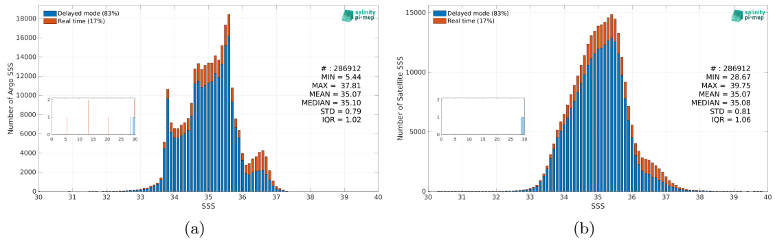
Figure 2: Histograms of SSS from Argo (a) and SMOS SSS L3 v9 - 9 Days (CATDS-CEC-LOCEAN) (b) considering all match-up pairs per bins of 0.1 over the Indian Ocean Pi-MEP region and for the full satellite product period.
