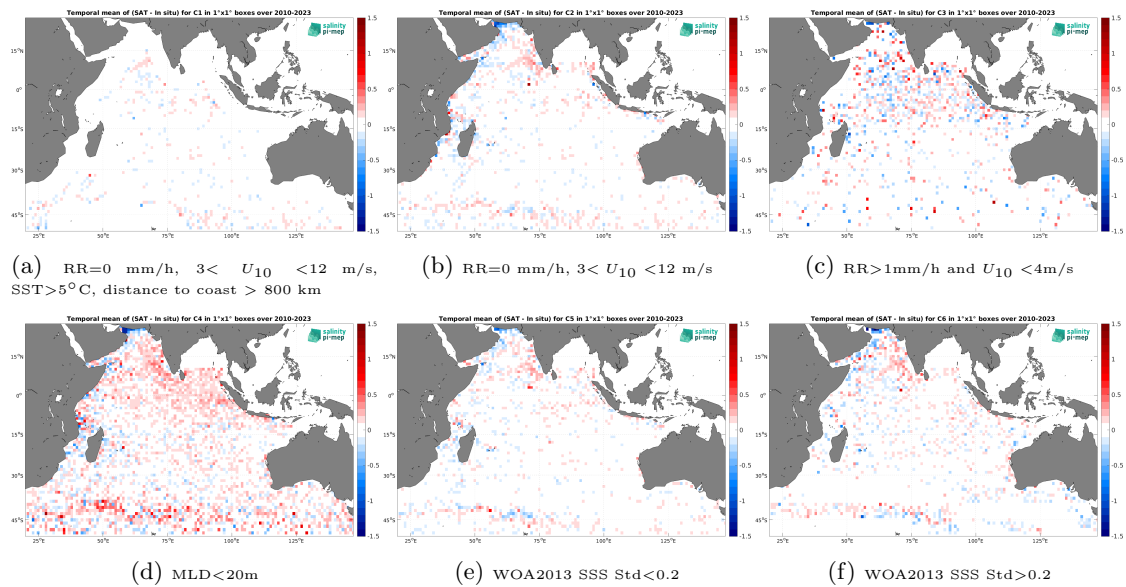
Figure 12: Temporal mean gridded over spatial boxes of size 1^\circ \times 1^\circ of \Delta SSS (SMOS SSS L3 v9 - 9 Days (CATDS-CEC-LOCEAN) - Argo) for 6 different subdatasets corresponding to:RR=0 mm/h, 3 < U_{10} < 12 m/s, SST >5^\circ C, distance to coast > 800 km (a), RR=0 mm/h, 3 < U_{10} < 12 m/s (b), RR >1 mm/h and U_{10} < 4 m/s (c),MLD <20 m (d),WOA2013 SSS Std <0.2 (e),WOA2013 SSS Std >0.2 (f).
