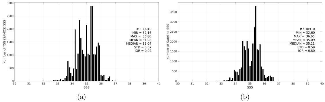
Figure 2: Histograms of SSS from TSG (SAMOS) (a) and SMOS SSS L3 v9 - 18 Days (CATDS-CEC-LOCEAN) (b) considering all match-up pairs per bins of 0.1 over the Indian Ocean Pi-MEP region and for the full satellite product period.
