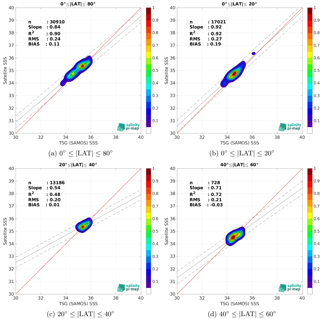
Figure 9: Contour maps of the concentration of SMOS SSS L3 v9 - 18 Days (CATDS-CEC-LOCEAN) SSS (y-axis) versus TSG (SAMOS) SSS (x-axis) at match-up pairs for different latitude bands. For each plot, the red line shows x=y . The black thin and dashed lines indicate a linear fit through the data cloud and the \pm 95\% confidence levels, respectively. The number match-up pairs n , the slope and R^2 coefficient of the linear fit, the root mean square (RMS) and the mean bias between satellite and in situ data are indicated for each latitude band in each plots.
