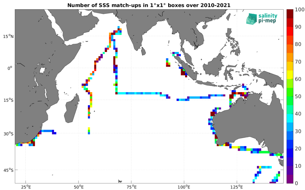
Figure 4: Number of SSS match-ups between TSG (SAMOS) SSS and the SMOS SSS L3 v9 - 18 Days (CATDS-CEC-LOCEAN) SSS product for the Indian Ocean Pi-MEP region over 1^\circ \times 1^\circ boxes and for the full satellite product period.
