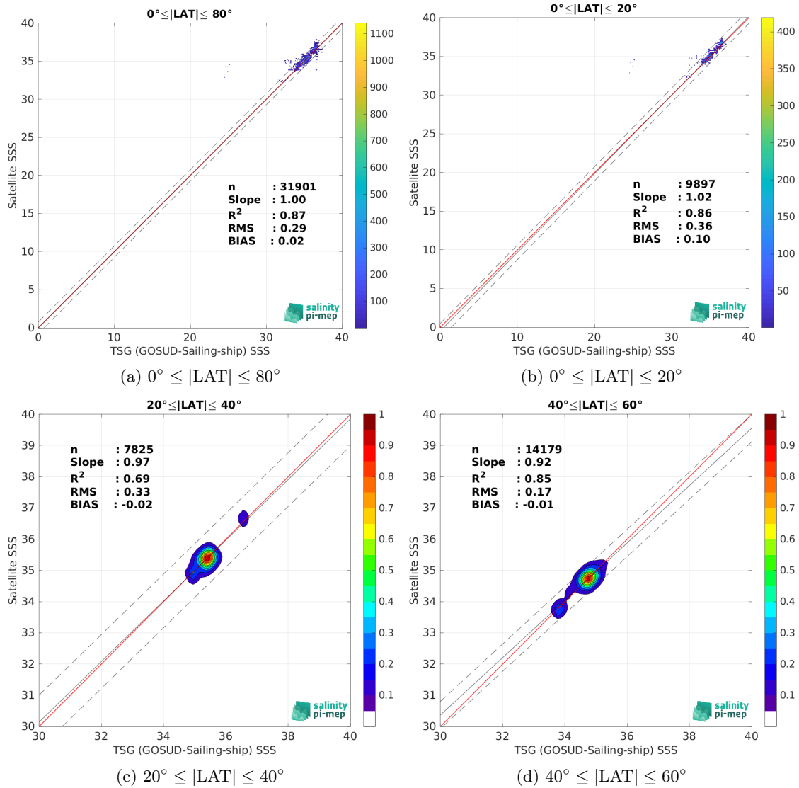
Figure 9: Contour maps of the concentration of SMOS SSS L3 v9 - 18 Days (CATDS-CEC-LOCEAN) SSS ( y -axis) versus TSG (GOSUD-Sailing-ship) SSS ( x -axis) at match-up pairs for different latitude bands. For each plot, the red line shows x=y . The black thin and dashed lines indicate a linear fit through the data cloud and the \pm 95\% confidence levels, respectively. The number match-up pairs n , the slope and R^2 coefficient of the linear fit, the root mean square (RMS) and the mean bias between satellite and in situ data are indicated for each latitude band in each plots.
