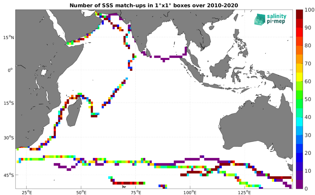
Figure 4: Number of SSS match-ups between TSG (GOSUD-Sailing-ship) SSS and the SMOS SSS L3 v9 - 18 Days (CATDS-CEC-LOCEAN) SSS product for the Indian Ocean Pi-MEP region over 1^{\circ} \times 1^{\circ} boxes and for the full satellite product period.
