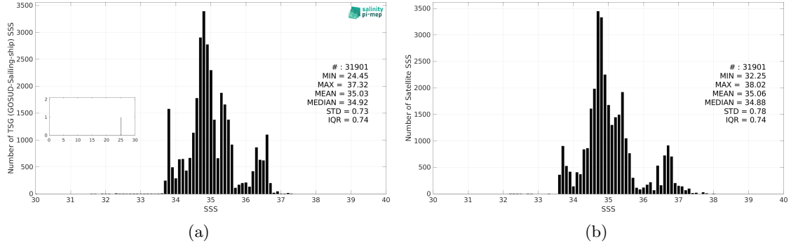
Figure 2: Histograms of SSS from TSG (GOSUD-Sailing-ship) (a) and SMOS SSS L3 v9 - 18 Days (CATDS-CEC-LOCEAN) (b) considering all match-up pairs per bins of 0.1 over the Indian Ocean Pi-MEP region and for the full satellite product period.
