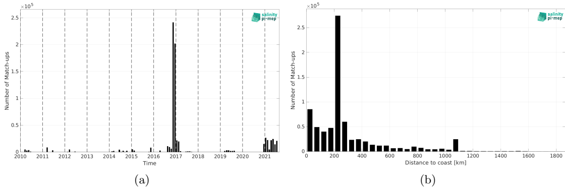
Figure 2: Number of match-ups between TSG (GOSUD-Research-vessel) and SMOS SSS L3 v9 - 18 Days (CATDS-CEC-LOCEAN) SSS as a function of time (a) and as function of the distance to coast (b) over the Indian Ocean Pi-MEP region and for the full satellite product period.
