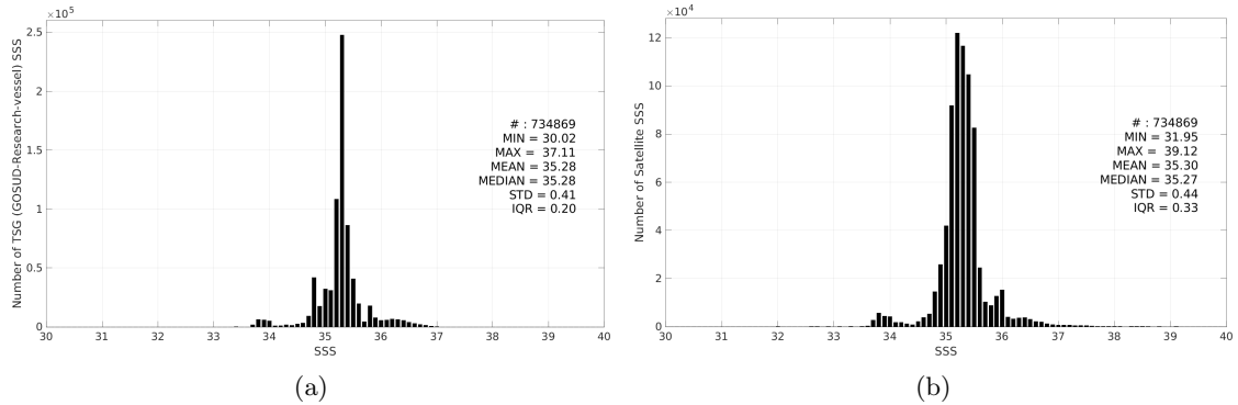
Figure 3: Histograms of SSS from TSG (GOSUD-Research-vessel) (a) and SMOS SSS L3 v9 - 18 Days (CATDS-CEC-LOCEAN) (b) considering all match-up pairs per bins of 0.1 over the Indian Ocean Pi-MEP region and for the full satellite product period.
