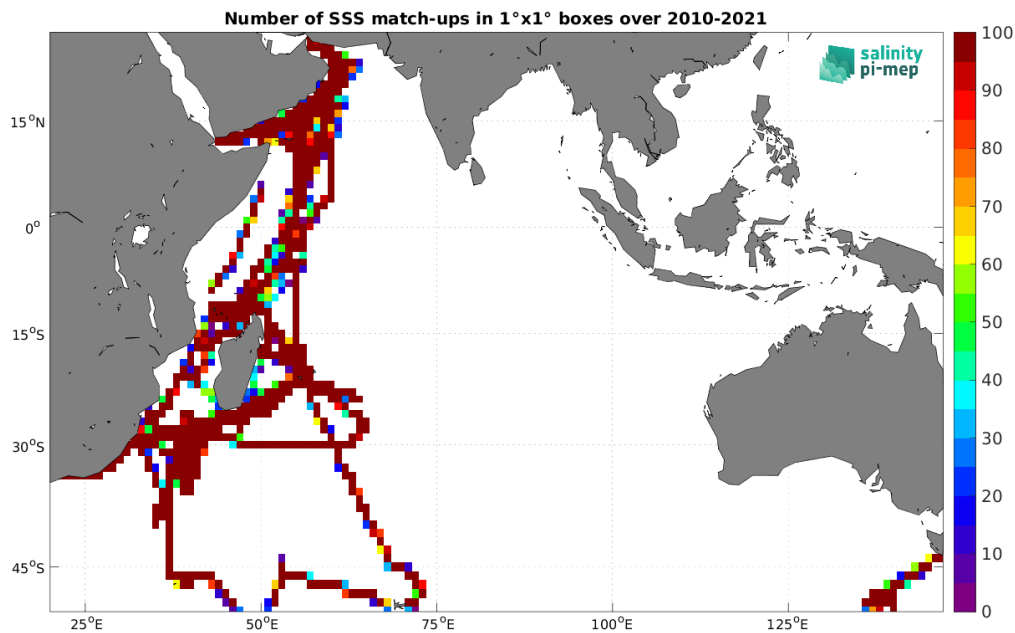
Figure 5: Number of SSS match-ups between TSG (GOSUD-Research-vessel) SSS and the SMOS SSS L3 v9 - 18 Days (CATDS-CEC-LOCEAN) SSS product for the Indian Ocean Pi-MEP region over 1^\circ \times 1^\circ boxes and for the full satellite product period.
