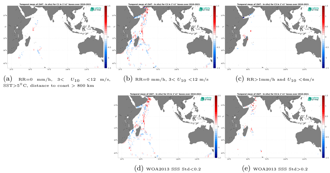
Figure 12: Temporal mean gridded over spatial boxes of size 1^\circ \times 1^\circ of \Delta SSS (SMOS SSS L3 v9 - 18 Days (CATDS-CEC-LOCEAN) - TSG (GOSUD-Research-vessel)) for 5 different subdatasets corresponding to:RR=0 mm/h, 3 < U_{10} < 12 m/s, SST >5^\circ C, distance to coast > 800 km (a), RR=0 mm/h, 3 < U_{10} < 12 m/s (b), RR >1 mm/h and U_{10} < 4 m/s (c), WOA2013 SSS Std <0.2 (d), WOA2013 SSS Std >0.2 (e).
