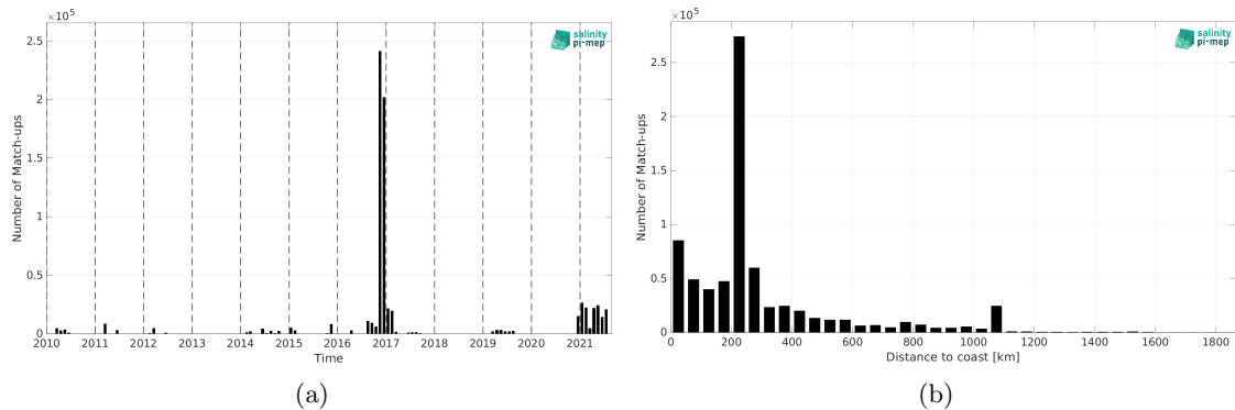
Figure 1: Number of match-ups between TSG (GOSUD-Research-vessel) and SMOS SSS L3 v9 - 18 Days (CATDS-CEC-LOCEAN) SSS as a function of time (a) and as function of the distance to coast (b) over the Indian Ocean Pi-MEP region and for the full satellite product period.
