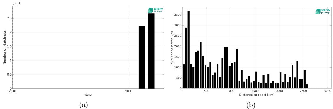
Figure 2: Number of match-ups between TSG (CSIC-UTM) and SMOS SSS L3 v9 - 18 Days (CATDS-CEC-LOCEAN) SSS as a function of time (a) and as function of the distance to coast (b) over the Indian Ocean Pi-MEP region and for the full satellite product period.
