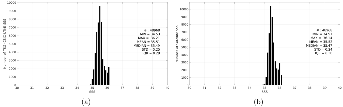
Figure 3: Histograms of SSS from TSG (CSIC-UTM) (a) and SMOS SSS L3 v9 - 18 Days (CATDS-CEC-LOCEAN) (b) considering all match-up pairs per bins of 0.1 over the Indian Ocean Pi-MEP region and for the full satellite product period.
