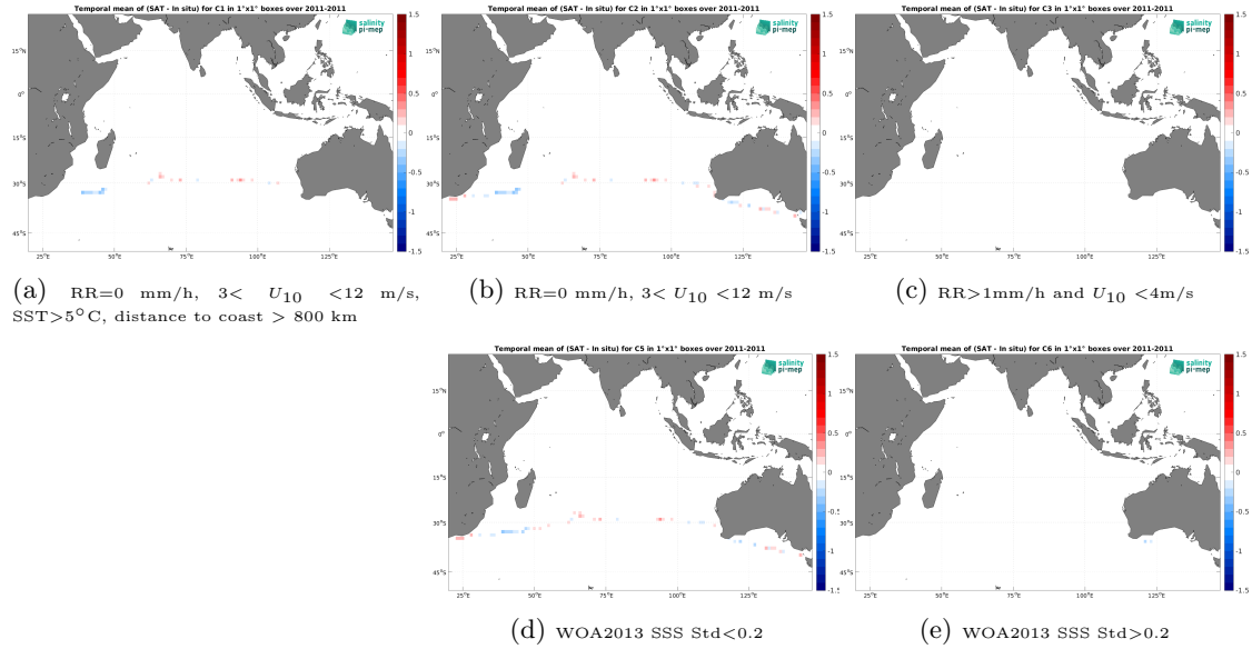
Figure 12: Temporal mean gridded over spatial boxes of size 1^{\circ}\times 1^{\circ} of \Delta\text{SSS} (SMOS SSS L3 v9 - 18 Days (CATDS-CEC-LOCEAN) - TSG (CSIC-UTM)) for 5 different subdatasets corresponding to:RR=0 mm/h, 3 < U_{10} < 12 m/s, SST >5^{\circ}\text{C} , distance to coast > 800 km (a), RR=0 mm/h, 3 < U_{10} < 12 m/s (b), RR >1 mm/h and U_{10} < 4 m/s (c), WOA2013 SSS Std <0.2 (d), WOA2013 SSS Std >0.2 (e).
