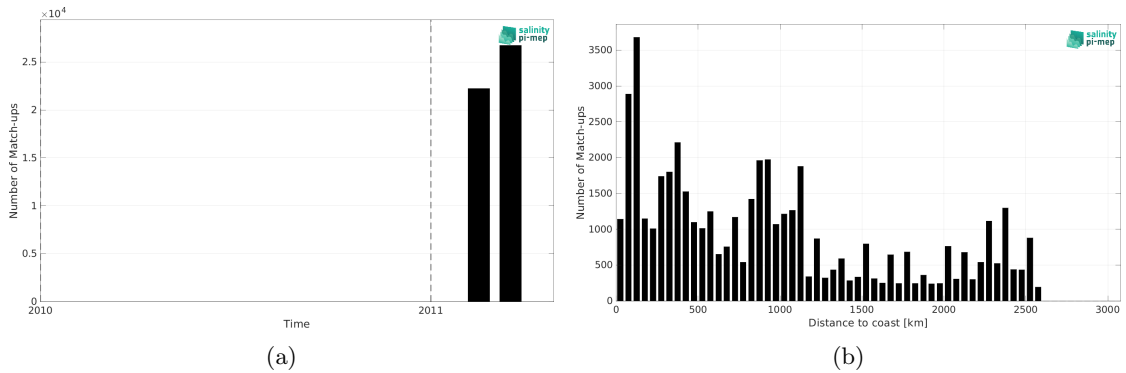
Figure 1: Number of match-ups between TSG (CSIC-UTM) and SMOS SSS L3 v9 - 18 Days (CATDS-CEC-LOCEAN) SSS as a function of time (a) and as function of the distance to coast (b) over the Indian Ocean Pi-MEP region and for the full satellite product period.
