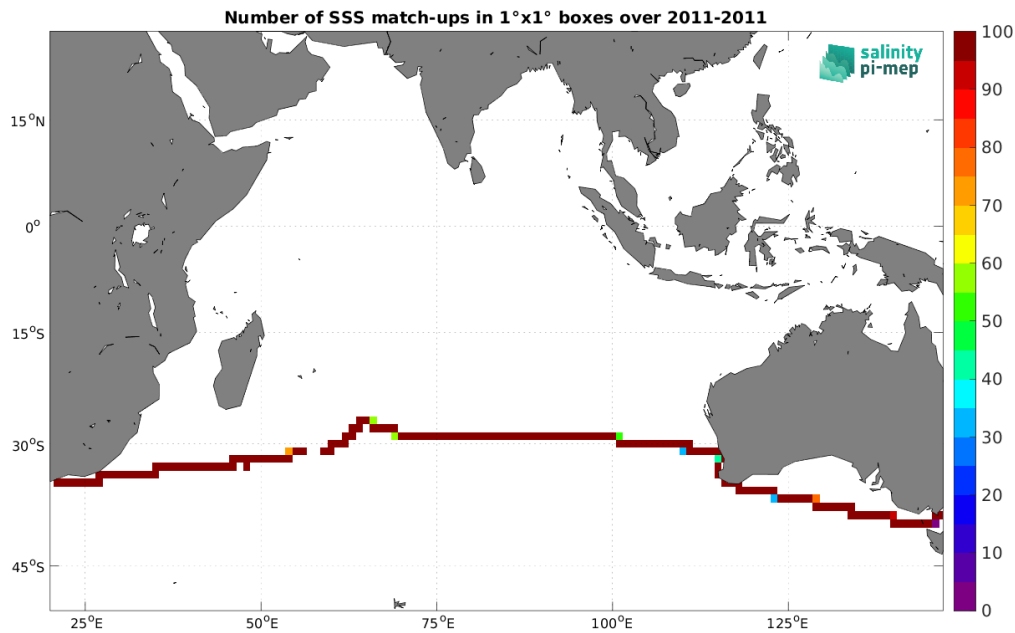
Figure 4: Number of SSS match-ups between TSG (CSIC-UTM) SSS and the SMOS SSS L3 v9 - 18 Days (CATDS-CEC-LOCEAN) SSS product for the Indian Ocean Pi-MEP region over 1^\circ \times 1^\circ boxes and for the full satellite product period.
