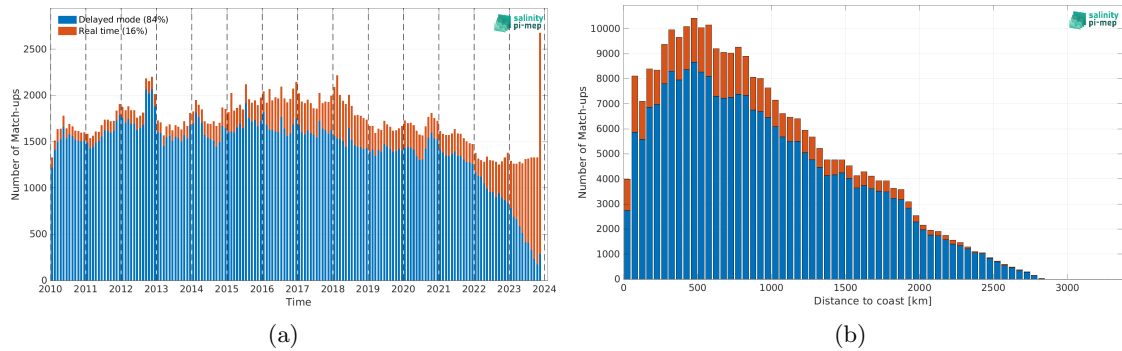
Figure 2: Number of match-ups between Argo and SMOS SSS L3 v9 - 18 Days (CATDS-CEC-LOCEAN) SSS as a function of time (a) and as function of the distance to coast (b) over the Indian Ocean Pi-MEP region and for the full satellite product period.
