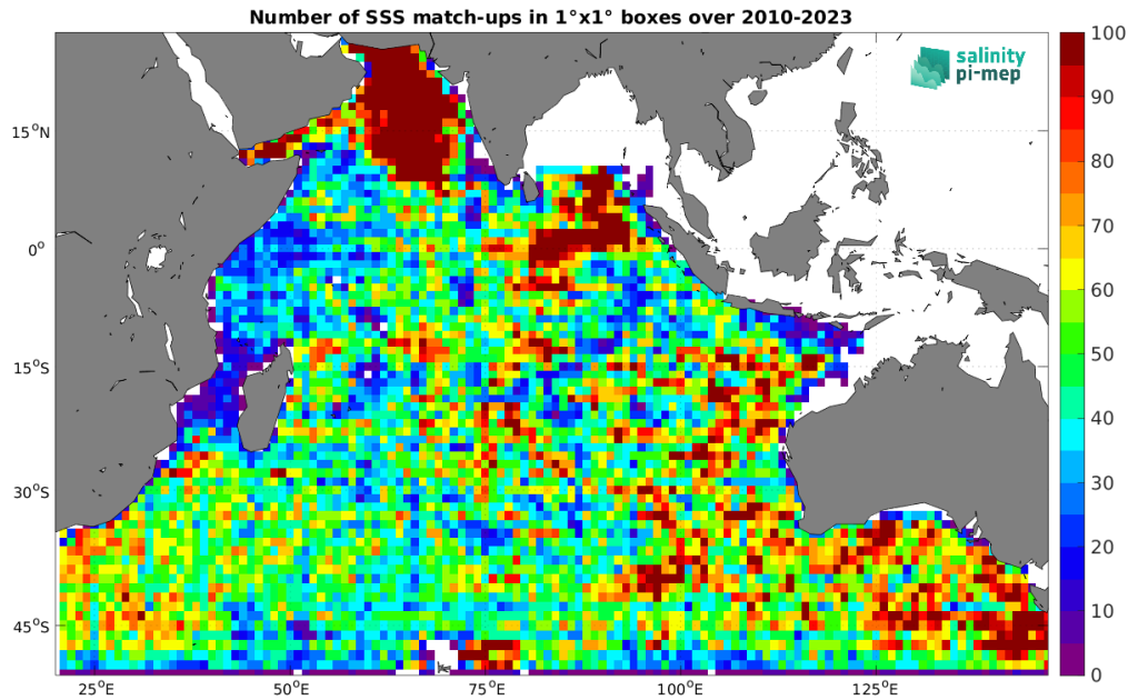
Figure 5: Number of SSS match-ups between Argo SSS and the SMOS SSS L3 v9 - 18 Days (CATDS-CEC-LOCEAN) SSS product for the Indian Ocean Pi-MEP region over 1^\circ \times 1^\circ boxes and for the full satellite product period.
