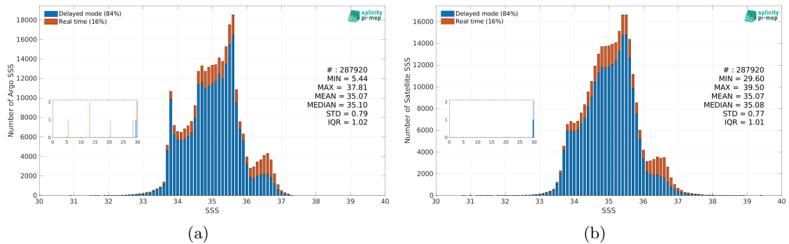
Figure 3: Histograms of SSS from Argo (a) and SMOS SSS L3 v9 - 18 Days (CATDS-CEC-LOCEAN) (b) considering all match-up pairs per bins of 0.1 over the Indian Ocean Pi-MEP region and for the full satellite product period.
