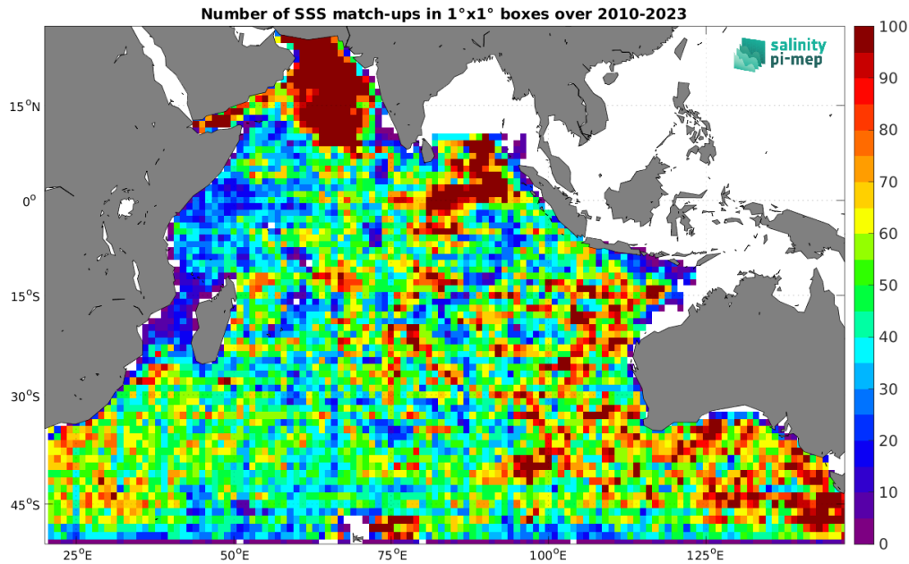
Figure 4: Number of SSS match-ups between Argo SSS and the SMOS SSS L3 v9 - 18 Days (CATDS-CEC-LOCEAN) SSS product for the Indian Ocean Pi-MEP region over 1^\circ \times 1^\circ boxes and for the full satellite product period.
