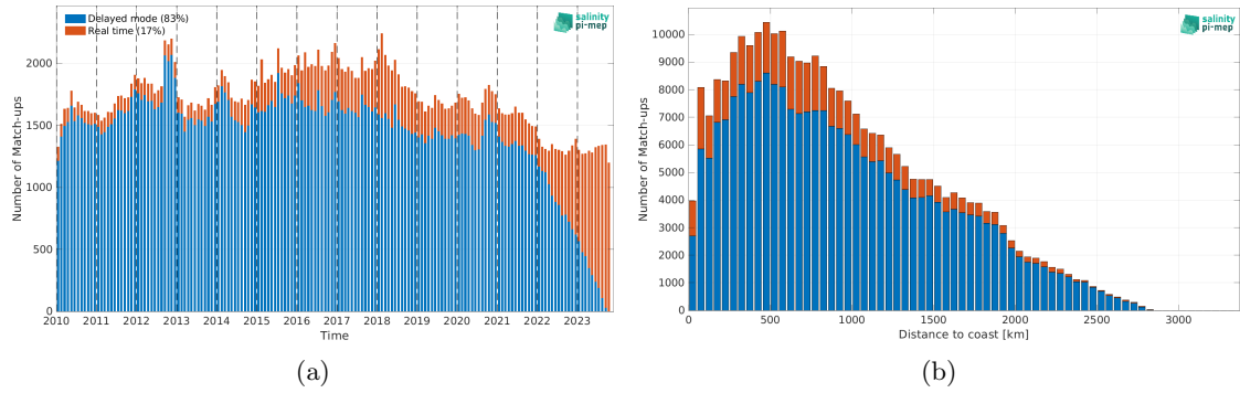
Figure 1: Number of match-ups between Argo and SMOS SSS L3 v9 - 18 Days (CATDS-CEC-LOCEAN) SSS as a function of time (a) and as function of the distance to coast (b) over the Indian Ocean Pi-MEP region and for the full satellite product period.
