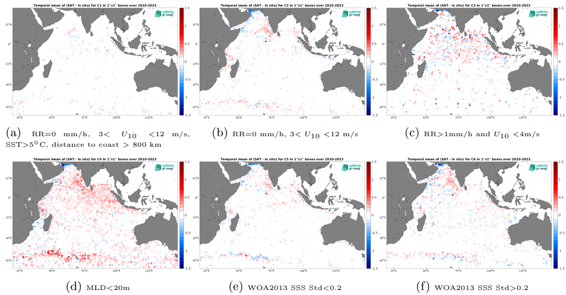
Figure 12: Temporal mean gridded over spatial boxes of size 1^\circ \times 1^\circ of \Delta SSS (SMOS SSS L3 v9 - 18 Days (CATDS-CEC-LOCEAN) - Argo) for 6 different subdatasets corresponding to:RR=0 mm/h, 3 < U_{10} < 12 m/s, SST >5^\circ C, distance to coast > 800 km (a), RR=0 mm/h, 3 < U_{10} < 12 m/s (b), RR >1 mm/h and U_{10} < 4 m/s (c),MLD <20 m (d),WOA2013 SSS Std <0.2 (e),WOA2013 SSS Std >0.2 (f).
