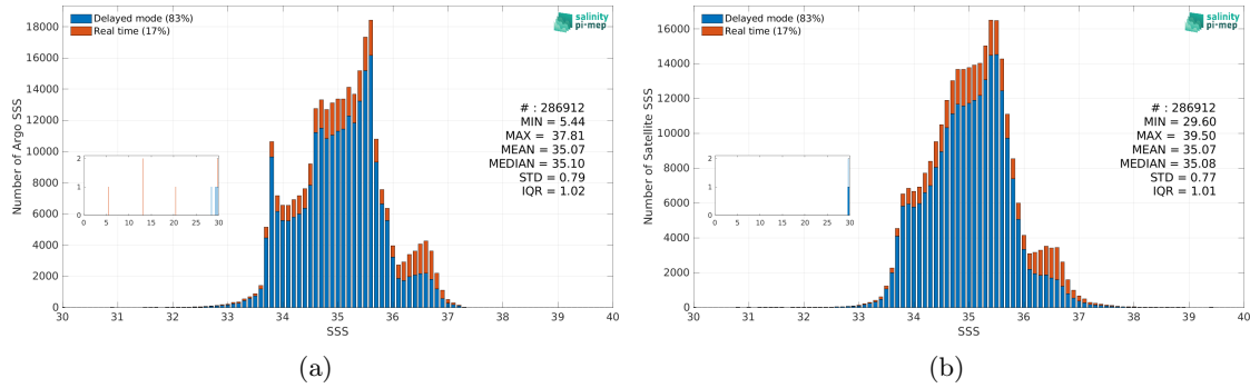
Figure 2: Histograms of SSS from Argo (a) and SMOS SSS L3 v9 - 18 Days (CATDS-CEC-LOCEAN) (b) considering all match-up pairs per bins of 0.1 over the Indian Ocean Pi-MEP region and for the full satellite product period.
