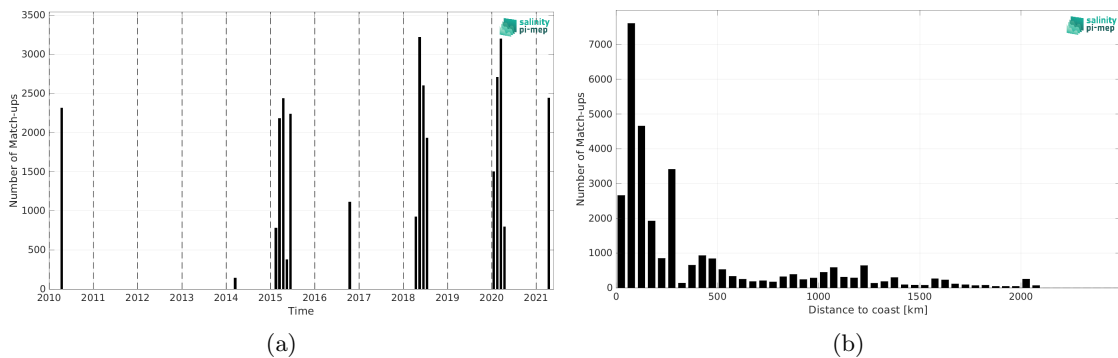
Figure 1: Number of match-ups between TSG (SAMOS) and SMOS SSS L3 v8 - 9 Days (CATDS-CEC-LOCEAN) SSS as a function of time (a) and as function of the distance to coast (b) over the Indian Ocean Pi-MEP region and for the full satellite product period.
