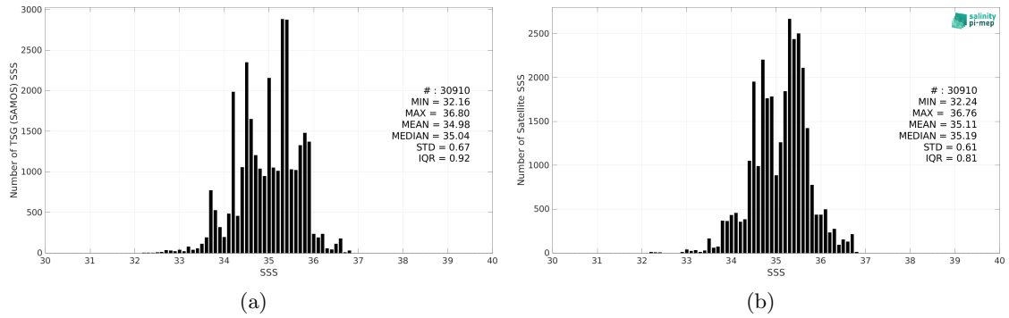
Figure 2: Histograms of SSS from TSG (SAMOS) (a) and SMOS SSS L3 v8 - 9 Days (CATDS-CEC-LOCEAN) (b) considering all match-up pairs per bins of 0.1 over the Indian Ocean Pi-MEP region and for the full satellite product period.
