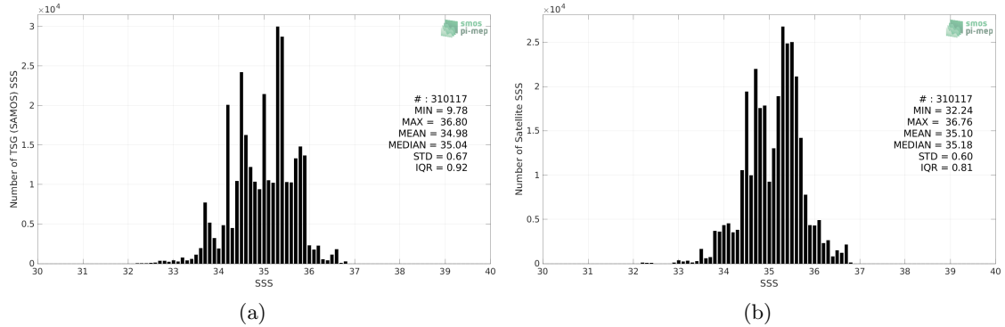
Figure 2: Histograms of SSS from TSG (SAMOS) (a) and SMOS SSS L3 v8 - 9 Days (CATDS-CECOS-LOCEAN) (b) considering all match-up pairs per bins of 0.1 over the Indian Ocean Pi-MEP region and for the full satellite product period.
