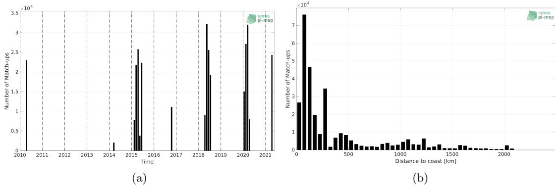
Figure 1: Number of match-ups between TSG (SAMOS) and SMOS SSS L3 v8 - 9 Days (CATDS-CECOS-LOCEAN) SSS as a function of time (a) and as function of the distance to coast (b) over the Indian Ocean Pi-MEP region and for the full satellite product period.
