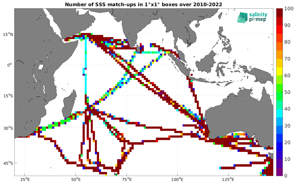
Figure 4: Number of SSS match-ups between TSG (LEGOS-DM) SSS and the SMOS SSS L3 v8 - 9 Days (CATDS-CEC-LOCEAN) SSS product for the Indian Ocean Pi-MEP region over 1^\circ \times 1^\circ boxes and for the full satellite product period.
