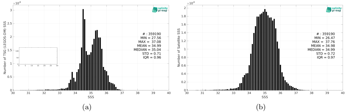
Figure 2: Histograms of SSS from TSG (LEGOS-DM) (a) and SMOS SSS L3 v8 - 9 Days (CATDS-CEC-LOCEAN) (b) considering all match-up pairs per bins of 0.1 over the Indian Ocean Pi-MEP region and for the full satellite product period.
