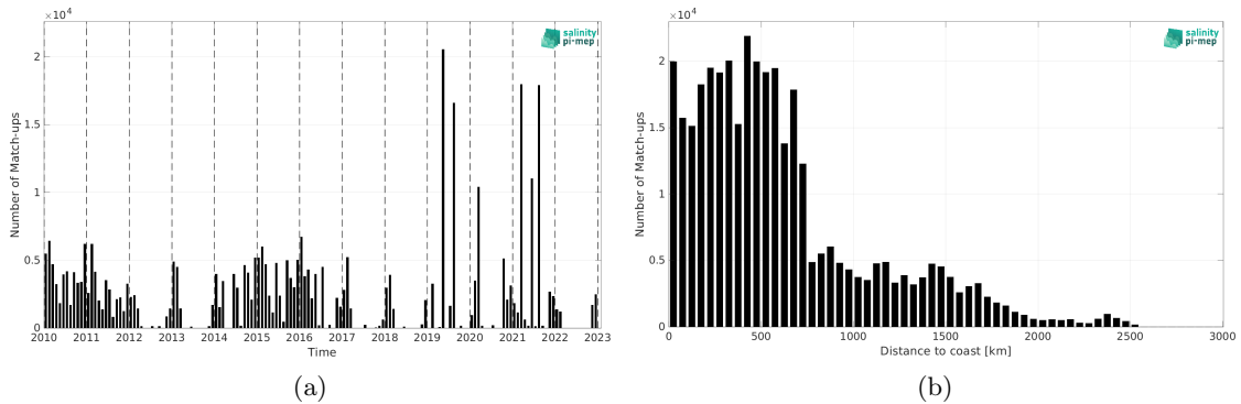
Figure 1: Number of match-ups between TSG (LEGOS-DM) and SMOS SSS L3 v8 - 9 Days (CATDS-CEC-LOCEAN) SSS as a function of time (a) and as function of the distance to coast (b) over the Indian Ocean Pi-MEP region and for the full satellite product period.
