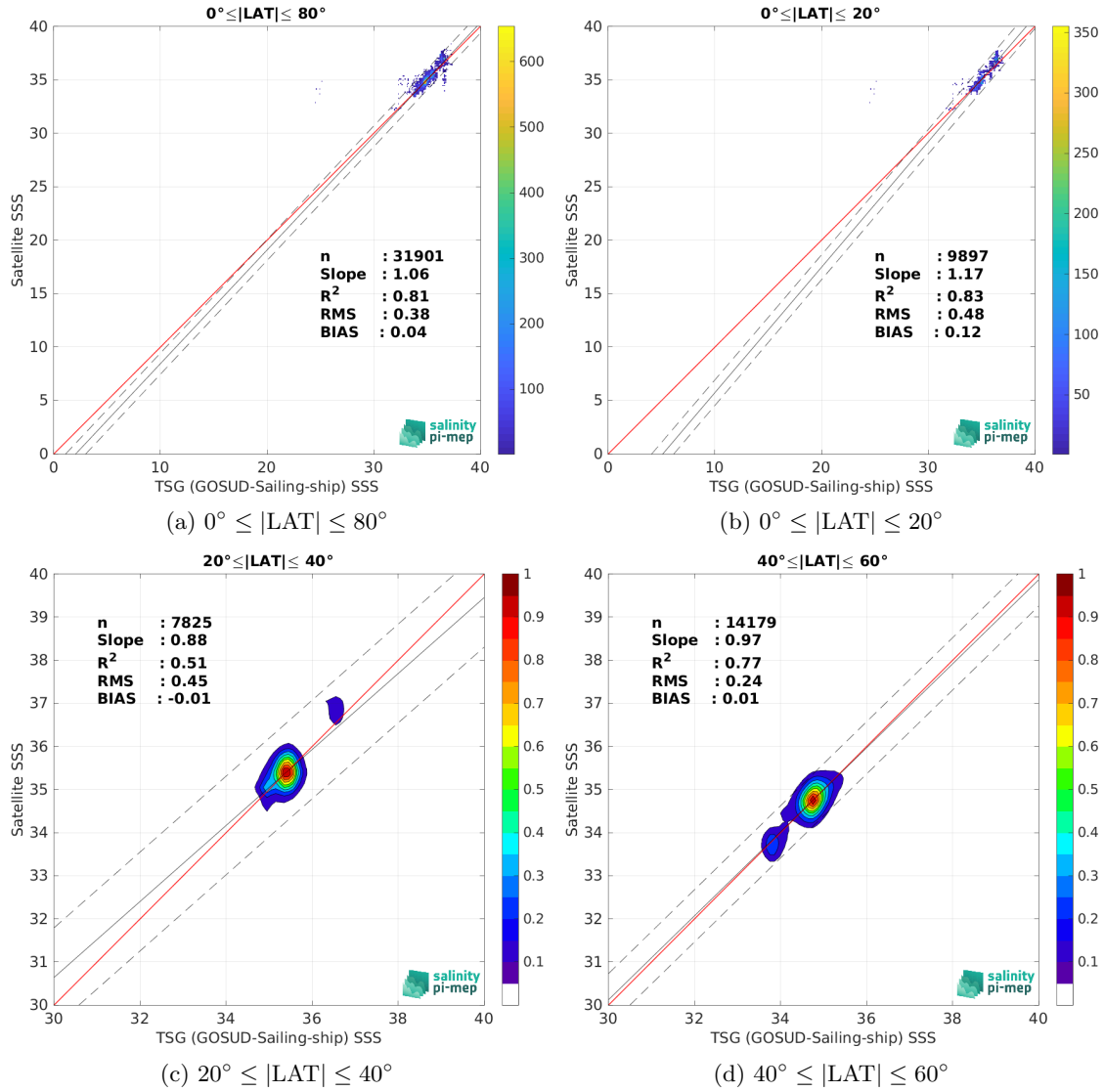
Figure 9: Contour maps of the concentration of SMOS SSS L3 v8 - 9 Days (CATDS-CEC-LOCEAN) SSS ( y -axis) versus TSG (GOSUD-Sailing-ship) SSS ( x -axis) at match-up pairs for different latitude bands. For each plot, the red line shows x=y . The black thin and dashed lines indicate a linear fit through the data cloud and the \pm 95\% confidence levels, respectively. The number match-up pairs n , the slope and R^2 coefficient of the linear fit, the root mean square (RMS) and the mean bias between satellite and in situ data are indicated for each latitude band in each plots.
