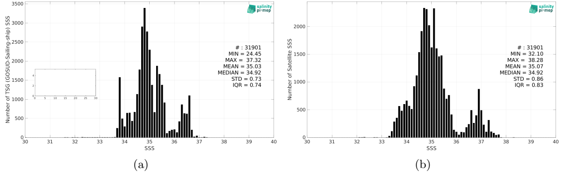
Figure 2: Histograms of SSS from TSG (GOSUD-Sailing-ship) (a) and SMOS SSS L3 v8 - 9 Days (CATDS-CEC-LOCEAN) (b) considering all match-up pairs per bins of 0.1 over the Indian Ocean Pi-MEP region and for the full satellite product period.
