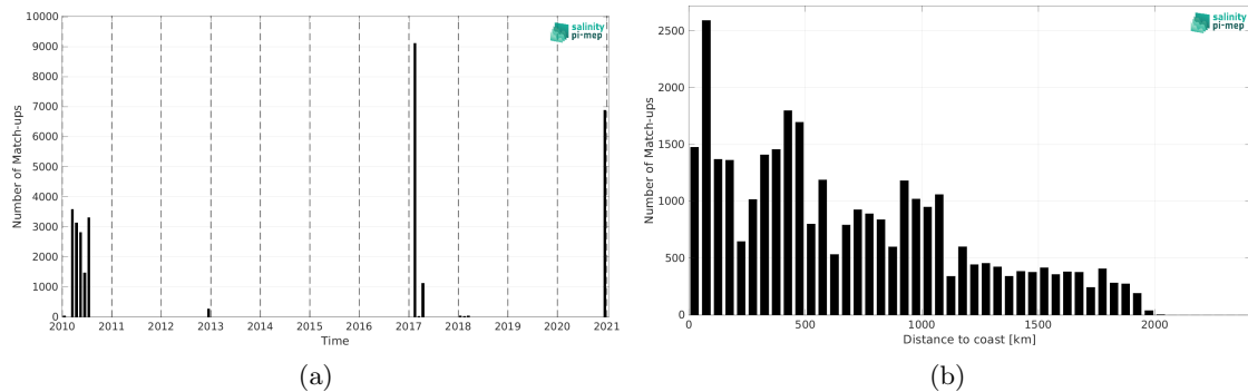
Figure 1: Number of match-ups between TSG (GOSUD-Sailing-ship) and SMOS SSS L3 v8 - 9 Days (CATDS-CEC-LOCEAN) SSS as a function of time (a) and as function of the distance to coast (b) over the Indian Ocean Pi-MEP region and for the full satellite product period.
