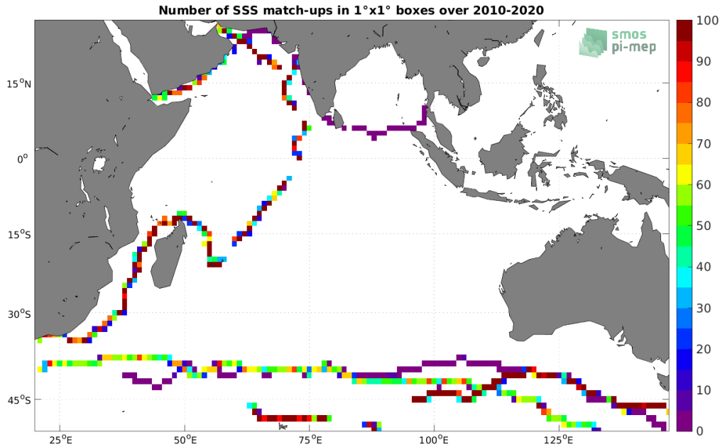
Figure 4: Number of SSS match-ups between TSG (GOSUD-Sailing-ship) SSS and the SMOS SSS L3 v8 - 9 Days (CATDS-CECOS-LOCEAN) SSS product for the Indian Ocean Pi-MEP region over 1^\circ \times 1^\circ boxes and for the full satellite product period.
