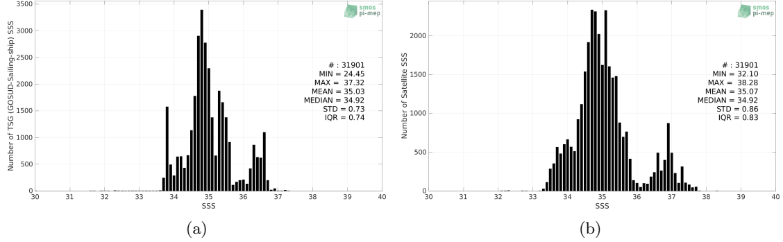
Figure 2: Histograms of SSS from TSG (GOSUD-Sailing-ship) (a) and SMOS SSS L3 v8 - 9 Days (CATDS-CECOS-LOCEAN) (b) considering all match-up pairs per bins of 0.1 over the Indian Ocean Pi-MEP region and for the full satellite product period.
