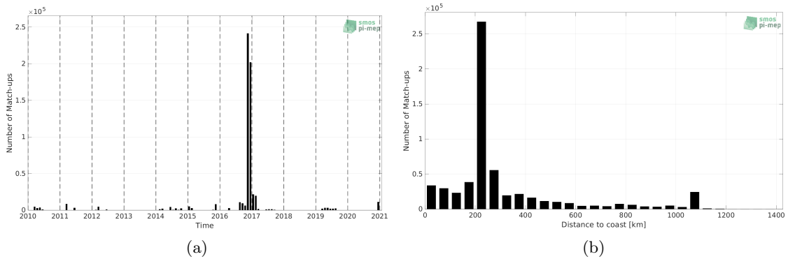
Figure 1: Number of match-ups between TSG (GOSUD-Research-vessel) and SMOS SSS L3 v8 - 9 Days (CATDS-CECOS-LOCEAN) SSS as a function of time (a) and as function of the distance to coast (b) over the Indian Ocean Pi-MEP region and for the full satellite product period.
