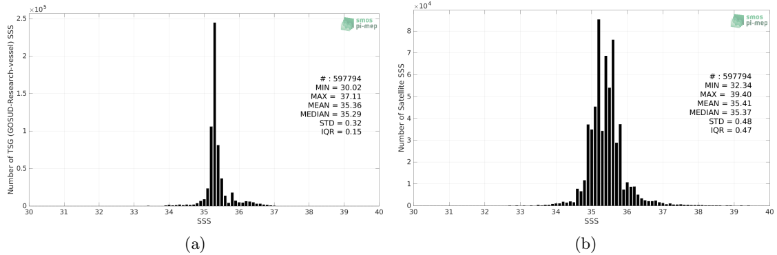
Figure 2: Histograms of SSS from TSG (GOSUD-Research-vessel) (a) and SMOS SSS L3 v8 - 9 Days (CATDS-CECOS-LOCEAN) (b) considering all match-up pairs per bins of 0.1 over the Indian Ocean Pi-MEP region and for the full satellite product period.
