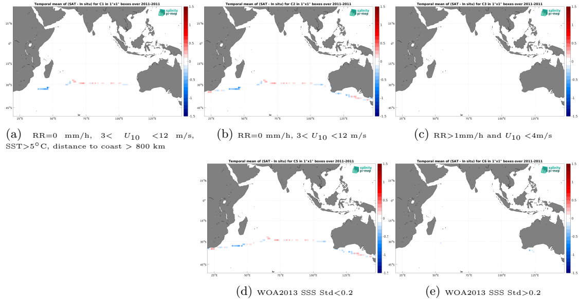
Figure 12: Temporal mean gridded over spatial boxes of size 1^{\circ}\times 1^{\circ} of \Delta\text{SSS} (SMOS SSS L3 v8 - 9 Days (CATDS-CEC-LOCEAN) - TSG (CSIC-UTM)) for 5 different subdatasets corresponding to:RR=0 mm/h, 3 < U_{10} < 12 m/s, SST >5^{\circ}\text{C} , distance to coast > 800 km (a), RR=0 mm/h, 3 < U_{10} < 12 m/s (b), RR >1 mm/h and U_{10} < 4 m/s (c), WOA2013 SSS Std <0.2 (d), WOA2013 SSS Std >0.2 (e).
