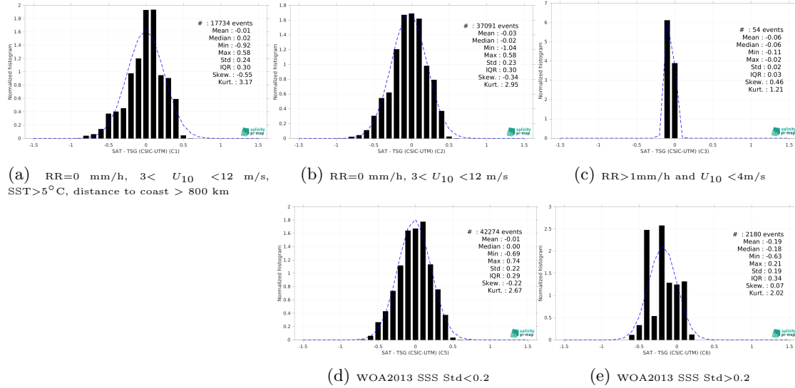
Figure 13: Normalized histogram of \Delta SSS (SMOS SSS L3 v8 - 9 Days (CATDS-CEC-LOCEAN) - TSG (CSIC-UTM)) for 5 different subdatasets corresponding to: RR=0 mm/h, 3 < U_{10} < 12 m/s, SST>5°C, distance to coast > 800 km (a), RR=0 mm/h, 3 < U_{10} < 12 m/s (b), RR>1mm/h and U_{10} < 4 m/s (c), WOA2013 SSS Std<0.2 (d), WOA2013 SSS Std>0.2 (e).
