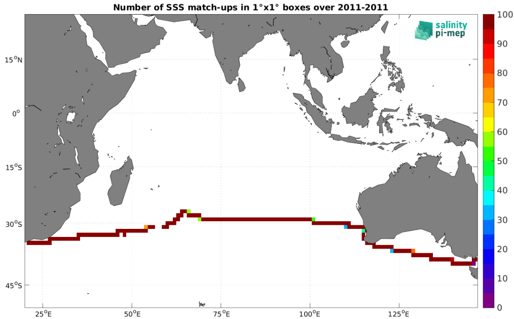
Figure 4: Number of SSS match-ups between TSG (CSIC-UTM) SSS and the SMOS SSS L3 v8 - 9 Days (CATDS-CEC-LOCEAN) SSS product for the Indian Ocean Pi-MEP region over 1^\circ \times 1^\circ boxes and for the full satellite product period.
