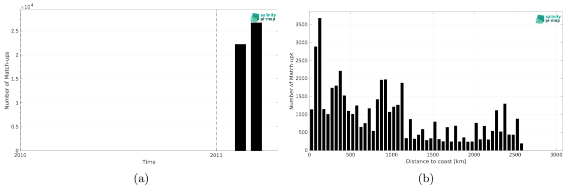
Figure 1: Number of match-ups between TSG (CSIC-UTM) and SMOS SSS L3 v8 - 9 Days (CATDS-CEC-LOCEAN) SSS as a function of time (a) and as function of the distance to coast (b) over the Indian Ocean Pi-MEP region and for the full satellite product period.
