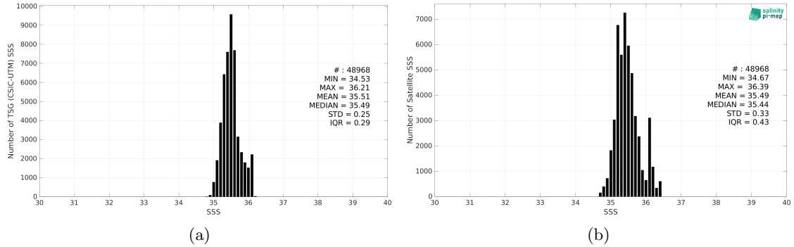
Figure 2: Histograms of SSS from TSG (CSIC-UTM) (a) and SMOS SSS L3 v8 - 9 Days (CATDS-CEC-LOCEAN) (b) considering all match-up pairs per bins of 0.1 over the Indian Ocean Pi-MEP region and for the full satellite product period.
