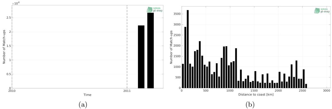
Figure 1: Number of match-ups between TSG (CSIC-UTM) and SMOS SSS L3 v8 - 9 Days (CATDS-CECOS-LOCEAN) SSS as a function of time (a) and as function of the distance to coast (b) over the Indian Ocean Pi-MEP region and for the full satellite product period.
