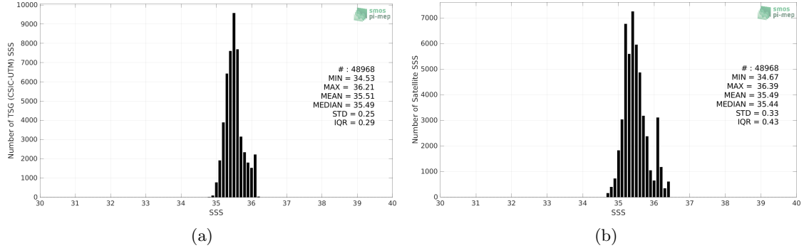
Figure 2: Histograms of SSS from TSG (CSIC-UTM) (a) and SMOS SSS L3 v8 - 9 Days (CATDS-CECOS-LOCEAN) (b) considering all match-up pairs per bins of 0.1 over the Indian Ocean Pi-MEP region and for the full satellite product period.
