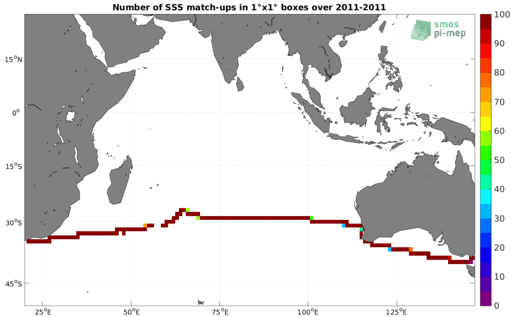
Figure 4: Number of SSS match-ups between TSG (CSIC-UTM) SSS and the SMOS SSS L3 v8 - 9 Days (CATDS-CECOS-LOCEAN) SSS product for the Indian Ocean Pi-MEP region over 1^\circ \times 1^\circ boxes and for the full satellite product period.
