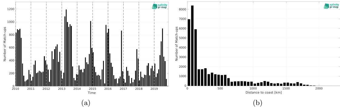
Figure 1: Number of match-ups between Marine mammals and SMOS SSS L3 v8 - 9 Days (CATDS-CEC-LOCEAN) SSS as a function of time (a) and as function of the distance to coast (b) over the Indian Ocean Pi-MEP region and for the full satellite product period.
