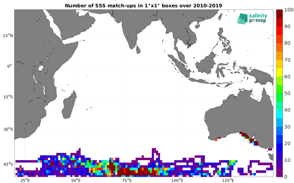
Figure 4: Number of SSS match-ups between Marine mammals SSS and the SMOS SSS L3 v8 - 9 Days (CATDS-CEC-LOCEAN) SSS product for the Indian Ocean Pi-MEP region over 1^\circ \times 1^\circ boxes and for the full satellite product period.
