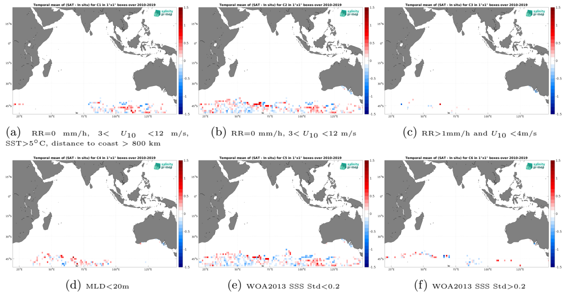
Figure 12: Temporal mean gridded over spatial boxes of size 1^{\circ}\times 1^{\circ} of \Delta\text{SSS} (SMOS SSS L3 v8 - 9 Days (CATDS-CEC-LOCEAN) - Marine mammals) for 6 different subdatasets corresponding to: \text{RR}=0 mm/h, 3 < U_{10} < 12 m/s, \text{SST} > 5^{\circ}\text{C} , distance to coast > 800 km (a), \text{RR}=0 mm/h, 3 < U_{10} < 12 m/s (b), \text{RR} > 1\text{mm/h} and U_{10} < 4\text{m/s} (c), \text{MLD} < 20\text{m} (d), WOA2013 SSS Std < 0.2 (e), WOA2013 SSS Std > 0.2 (f).
