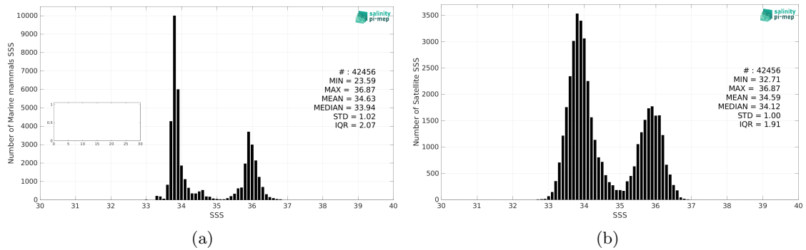
Figure 2: Histograms of SSS from Marine mammals (a) and SMOS SSS L3 v8 - 9 Days (CATDS-CEC-LOCEAN) (b) considering all match-up pairs per bins of 0.1 over the Indian Ocean Pi-MEP region and for the full satellite product period.
