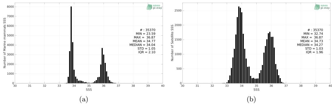
Figure 2: Histograms of SSS from Marine mammals (a) and SMOS SSS L3 v8 - 9 Days (CATDS-CECOS-LOCEAN) (b) considering all match-up pairs per bins of 0.1 over the Indian Ocean Pi-MEP region and for the full satellite product period.
