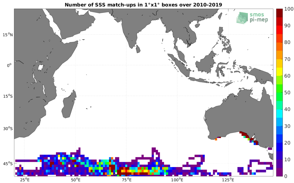
Figure 4: Number of SSS match-ups between Marine mammals SSS and the SMOS SSS L3 v8 - 9 Days (CATDS-CECOS-LOCEAN) SSS product for the Indian Ocean Pi-MEP region over 1^\circ \times 1^\circ boxes and for the full satellite product period.
