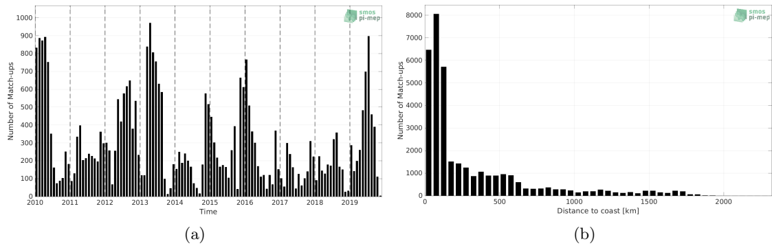
Figure 1: Number of match-ups between Marine mammals and SMOS SSS L3 v8 - 9 Days (CATDS-CECOS-LOCEAN) SSS as a function of time (a) and as function of the distance to coast (b) over the Indian Ocean Pi-MEP region and for the full satellite product period.
