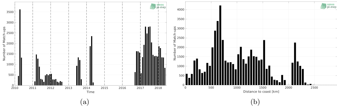
Figure 1: Number of match-ups between Surface drifters and SMOS SSS L3 v8 - 9 Days (CATDS-CECOS-LOCEAN) SSS as a function of time (a) and as function of the distance to coast (b) over the Indian Ocean Pi-MEP region and for the full satellite product period.
