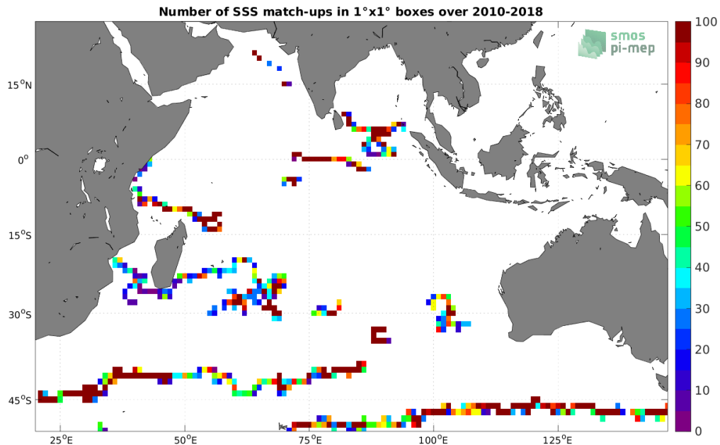
Figure 3: Number of SSS match-ups between Surface drifters SSS and the SMOS SSS L3 v8 - 9 Days (CATDS-CECOS-LOCEAN) SSS product for the Indian Ocean Pi-MEP region over 1^\circ \times 1^\circ boxes and for the full satellite product period.
