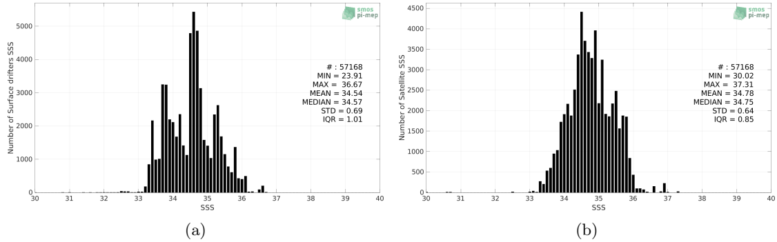
Figure 2: Histograms of SSS from Surface drifters (a) and SMOS SSS L3 v8 - 9 Days (CATDS-CECOS-LOCEAN) (b) considering all match-up pairs per bins of 0.1 over the Indian Ocean Pi-MEP region and for the full satellite product period.
