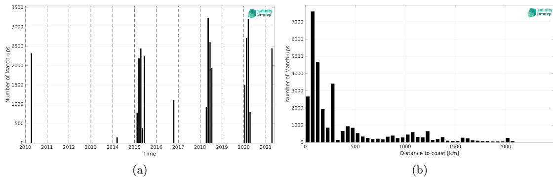
Figure 1: Number of match-ups between TSG (SAMOS) and SMOS SSS L3 v8 - 18 Days (CATDS-CEC-LOCEAN) SSS as a function of time (a) and as function of the distance to coast (b) over the Indian Ocean Pi-MEP region and for the full satellite product period.
