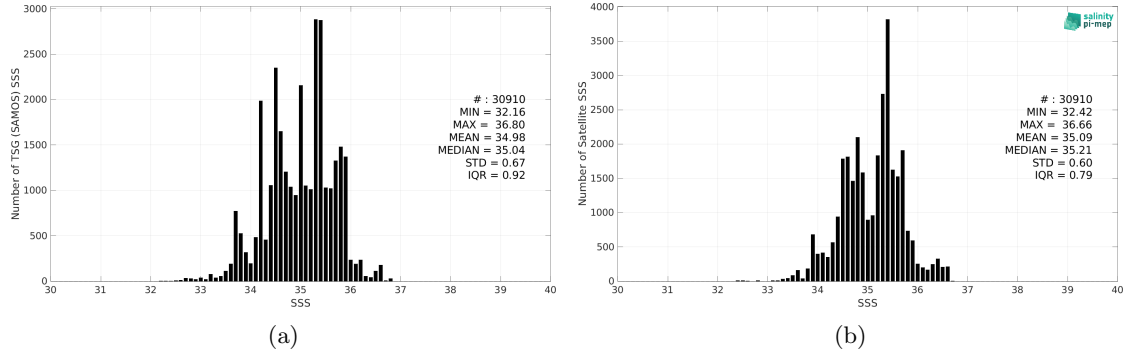
Figure 2: Histograms of SSS from TSG (SAMOS) (a) and SMOS SSS L3 v8 - 18 Days (CATDS-CEC-LOCEAN) (b) considering all match-up pairs per bins of 0.1 over the Indian Ocean Pi-MEP region and for the full satellite product period.
