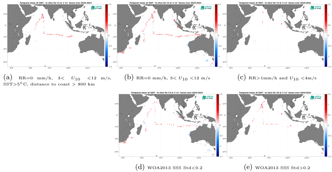
Figure 12: Temporal mean gridded over spatial boxes of size 1^\circ \times 1^\circ of \Delta SSS (SMOS SSS L3 v8 - 18 Days (CATDS-CEC-LOCEAN) - TSG (SAMOS)) for 5 different subdatasets corresponding to:RR=0 mm/h, 3 < U_{10} < 12 m/s, SST >5^\circ C, distance to coast > 800 km (a), RR=0 mm/h, 3 < U_{10} < 12 m/s (b), RR >1 mm/h and U_{10} < 4 m/s (c), WOA2013 SSS Std <0.2 (d), WOA2013 SSS Std >0.2 (e).
