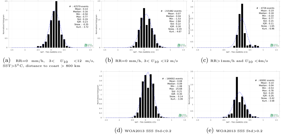
Figure 13: Normalized histogram of \Delta SSS (SMOS SSS L3 v8 - 18 Days (CATDS-CECOS-LOCEAN) - TSG (SAMOS)) for 5 different subdatasets corresponding to: RR=0 mm/h, 3 < U_{10} < 12 m/s, SST > 5°C, distance to coast > 800 km (a), RR=0 mm/h, 3 < U_{10} < 12 m/s (b), RR > 1mm/h and U_{10} < 4 m/s (c), WOA2013 SSS Std < 0.2 (d), WOA2013 SSS Std > 0.2 (e).
