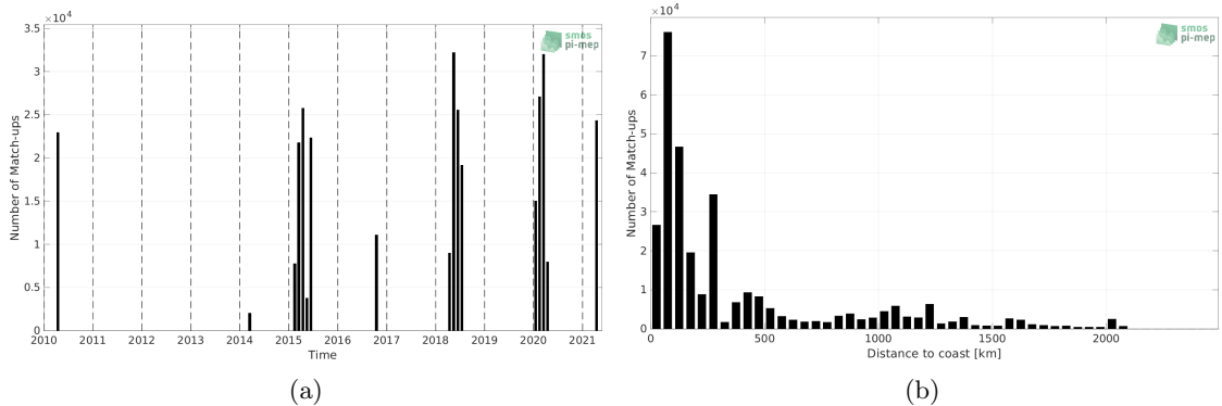
Figure 1: Number of match-ups between TSG (SAMOS) and SMOS SSS L3 v8 - 18 Days (CATDS-CECOS-LOCEAN) SSS as a function of time (a) and as function of the distance to coast (b) over the Indian Ocean Pi-MEP region and for the full satellite product period.
