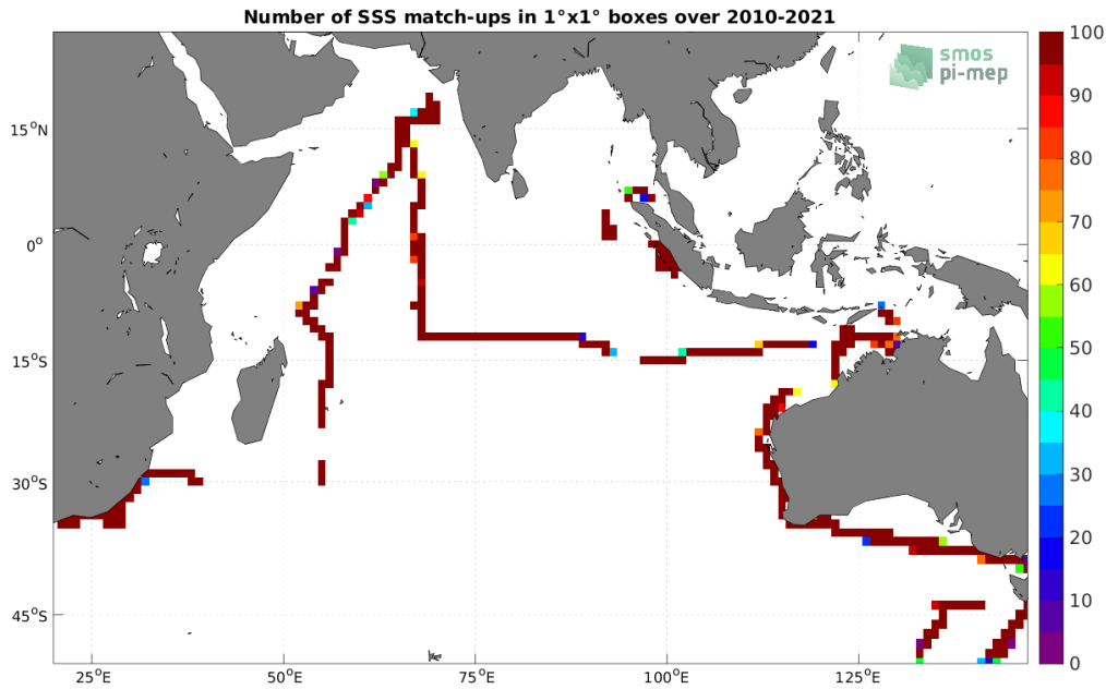
Figure 4: Number of SSS match-ups between TSG (SAMOS) SSS and the SMOS SSS L3 v8 - 18 Days (CATDS-CECOS-LOCEAN) SSS product for the Indian Ocean Pi-MEP region over 1^\circ \times 1^\circ boxes and for the full satellite product period.
