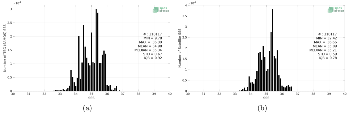
Figure 2: Histograms of SSS from TSG (SAMOS) (a) and SMOS SSS L3 v8 - 18 Days (CATDS-CECOS-LOCEAN) (b) considering all match-up pairs per bins of 0.1 over the Indian Ocean Pi-MEP region and for the full satellite product period.
