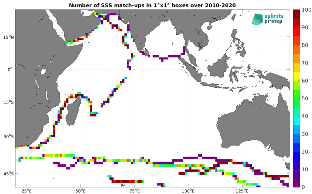
Figure 4: Number of SSS match-ups between TSG (GOSUD-Sailing-ship) SSS and the SMOS SSS L3 v8 - 18 Days (CATDS-CEC-LOCEAN) SSS product for the Indian Ocean Pi-MEP region over 1^\circ \times 1^\circ boxes and for the full satellite product period.
