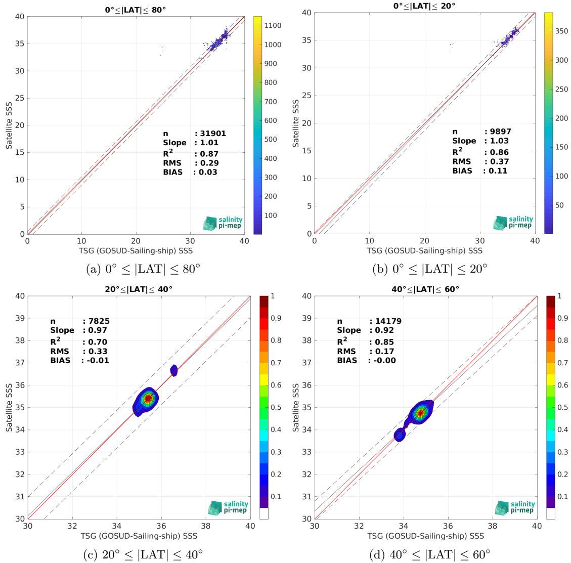
Figure 9: Contour maps of the concentration of SMOS SSS L3 v8 - 18 Days (CATDS-CEC-LOCEAN) SSS ( y -axis) versus TSG (GOSUD-Sailing-ship) SSS ( x -axis) at match-up pairs for different latitude bands. For each plot, the red line shows x=y . The black thin and dashed lines indicate a linear fit through the data cloud and the \pm 95\% confidence levels, respectively. The number match-up pairs n , the slope and R^2 coefficient of the linear fit, the root mean square (RMS) and the mean bias between satellite and in situ data are indicated for each latitude band in each plots.
