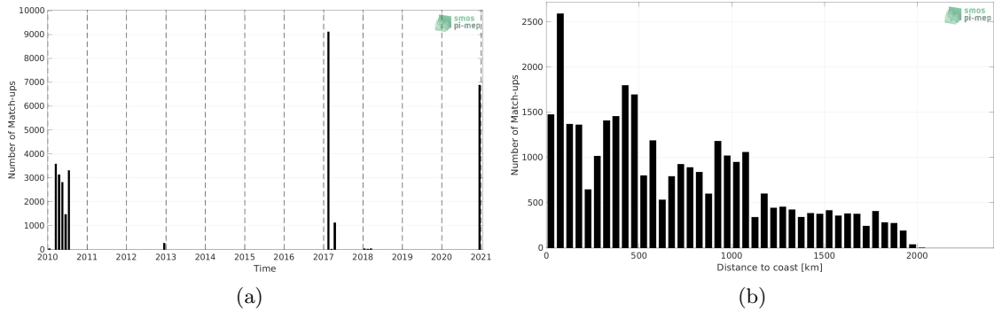
Figure 1: Number of match-ups between TSG (GOSUD-Sailing-ship) and SMOS SSS L3 v8 - 18 Days (CATDS-CECOS-LOCEAN) SSS as a function of time (a) and as function of the distance to coast (b) over the Indian Ocean Pi-MEP region and for the full satellite product period.
