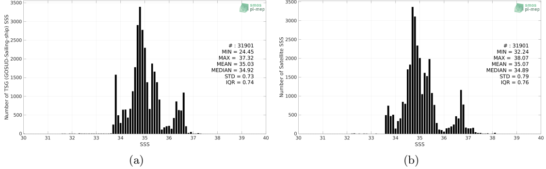
Figure 2: Histograms of SSS from TSG (GOSUD-Sailing-ship) (a) and SMOS SSS L3 v8 - 18 Days (CATDS-CECOS-LOCEAN) (b) considering all match-up pairs per bins of 0.1 over the Indian Ocean Pi-MEP region and for the full satellite product period.
