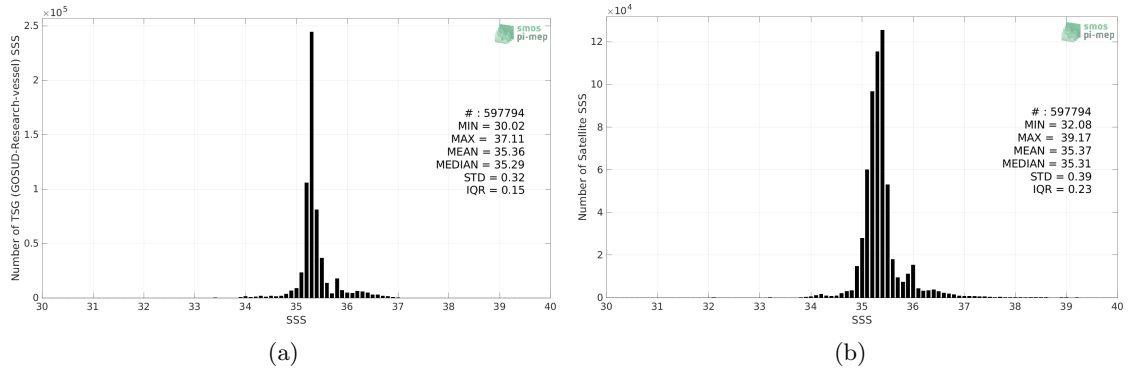
Figure 2: Histograms of SSS from TSG (GOSUD-Research-vessel) (a) and SMOS SSS L3 v8 - 18 Days (CATDS-CECOS-LOCEAN) (b) considering all match-up pairs per bins of 0.1 over the Indian Ocean Pi-MEP region and for the full satellite product period.
