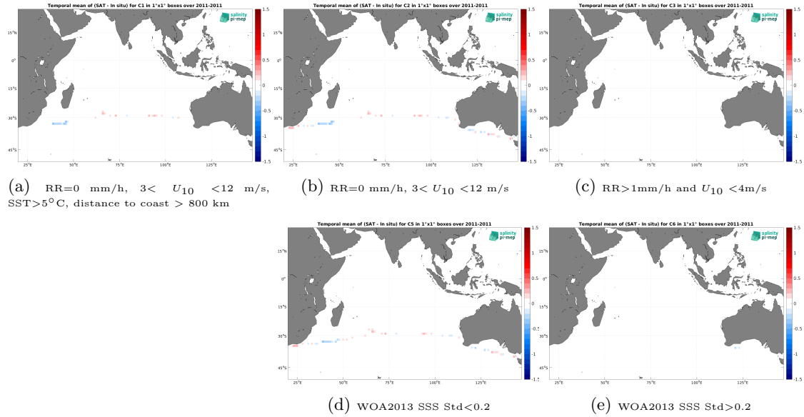
Figure 12: Temporal mean gridded over spatial boxes of size 1^{\circ}\times 1^{\circ} of \Delta\text{SSS} (SMOS SSS L3 v8 - 18 Days (CATDS-CEC-LOCEAN) - TSG (CSIC-UTM)) for 5 different subdatasets corresponding to:RR=0 mm/h, 3 < U_{10} < 12 m/s, SST >5^{\circ}\text{C} , distance to coast > 800 km (a), RR=0 mm/h, 3 < U_{10} < 12 m/s (b), RR >1 mm/h and U_{10} < 4 m/s (c), WOA2013 SSS Std <0.2 (d), WOA2013 SSS Std >0.2 (e).
