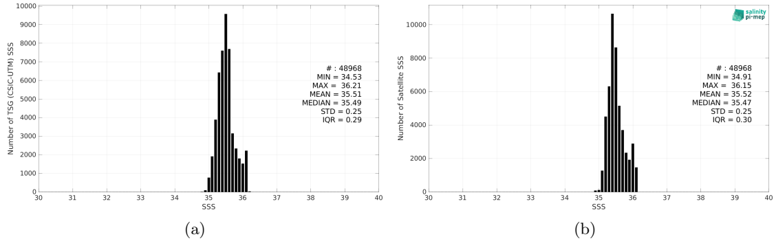
Figure 2: Histograms of SSS from TSG (CSIC-UTM) (a) and SMOS SSS L3 v8 - 18 Days (CATDS-CEC-LOCEAN) (b) considering all match-up pairs per bins of 0.1 over the Indian Ocean Pi-MEP region and for the full satellite product period.
