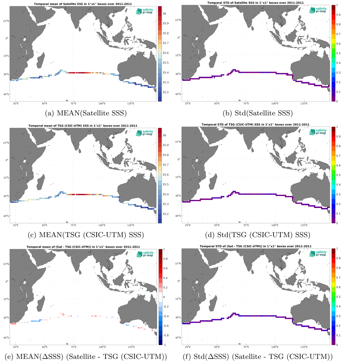
Figure 6: Temporal mean (left) and Std (right) of SSS from SMOS SSS L3 v8 - 18 Days (CATDS-CEC-LOCEAN) (top), TSG (CSIC-UTM) (middle), and of \Delta SSS (Satellite - TSG (CSIC-UTM)). Only match-up pairs are used to generate these maps.
