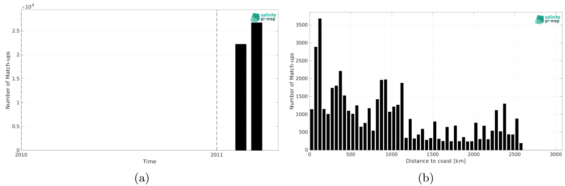
Figure 1: Number of match-ups between TSG (CSIC-UTM) and SMOS SSS L3 v8 - 18 Days (CATDS-CEC-LOCEAN) SSS as a function of time (a) and as function of the distance to coast (b) over the Indian Ocean Pi-MEP region and for the full satellite product period.
